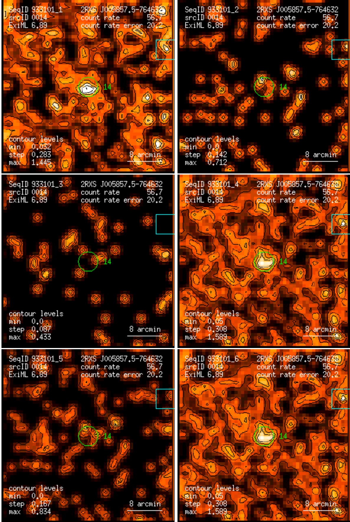
Figure 14: RASS 933101: detection 0014: band rate images, Gaussian filter: (1) PSPC channels 11 – 41, (2) 52 – 90, (3) 91 – 201, (4) 11 – 235, (5) 52 – 201, (6) 11 – 201. Broad band rates in counts/ks. Band rate contour levels in counts/ks/arcmin 2 .
