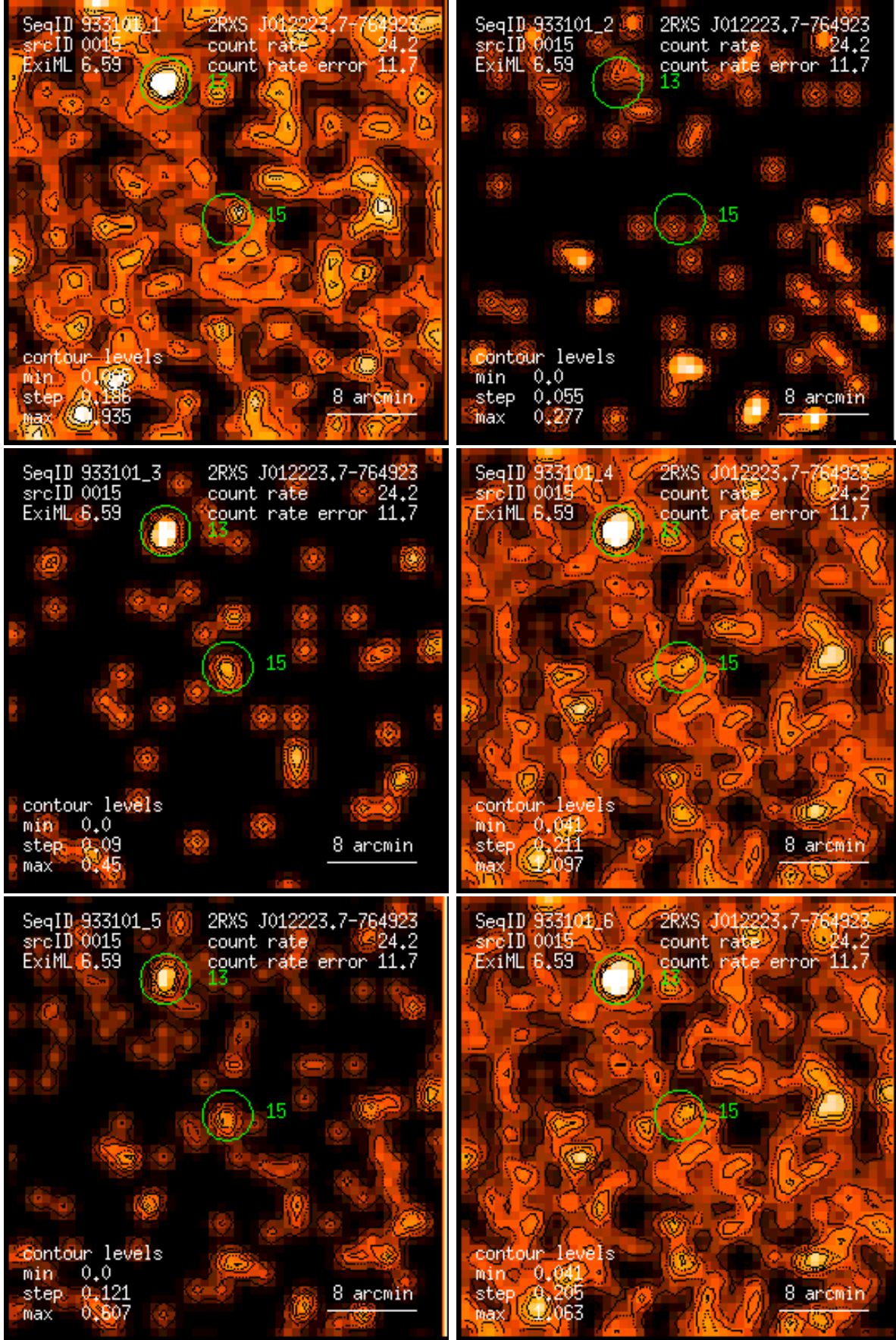
Figure 15: RASS 933101: detection 0015: band rate images, Gaussian filter: (1) PSPC channels 11 – 41, (2) 52 – 90, (3) 91 – 201, (4) 11 – 235, (5) 52 – 201, (6) 11 – 201. Broad band rates in counts/ks. Band rate contour levels in counts/ks/arcmin 2 .
