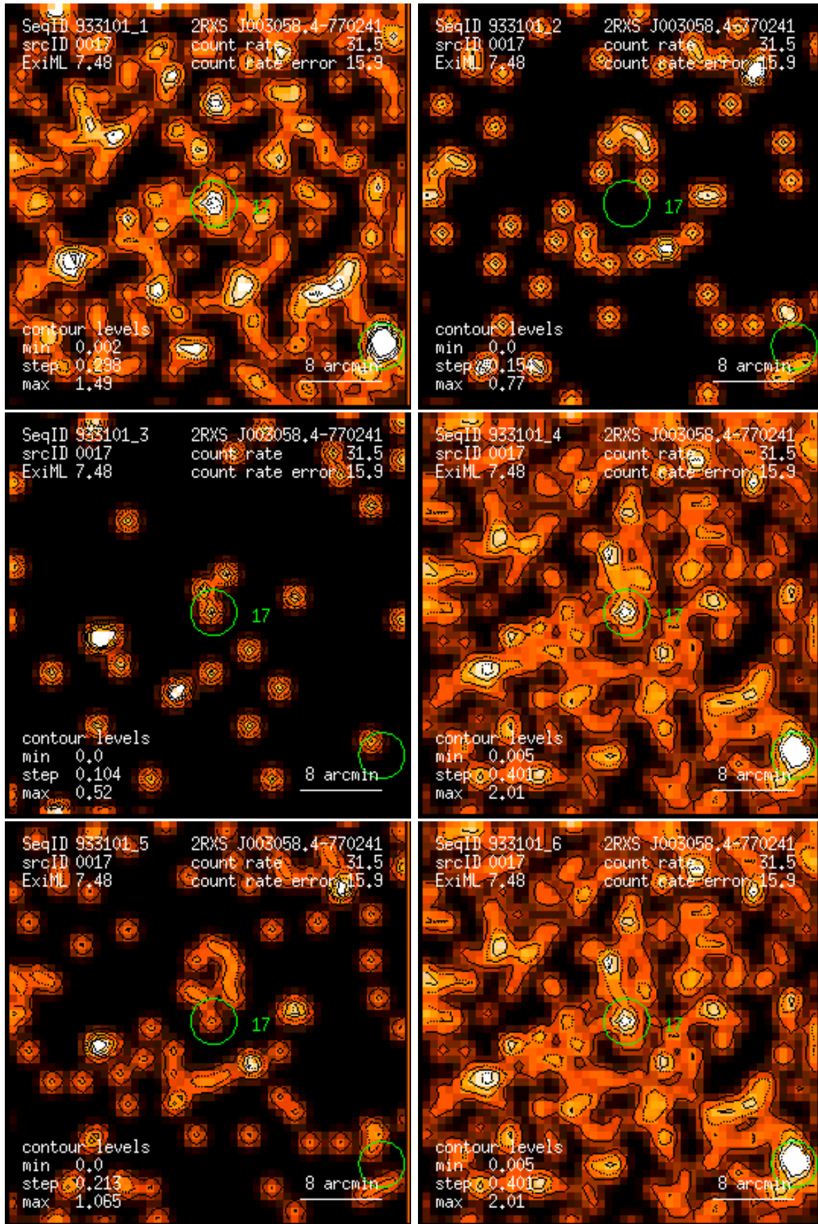
Figure 17: RASS 933101: detection 0017: band rate images, Gaussian filter: (1) PSPC channels 11 – 41, (2) 52 – 90, (3) 91 – 201, (4) 11 – 235, (5) 52 – 201, (6) 11 – 201. Broad band rates in counts/ks. Band rate contour levels in counts/ks/arcmin 2 .
