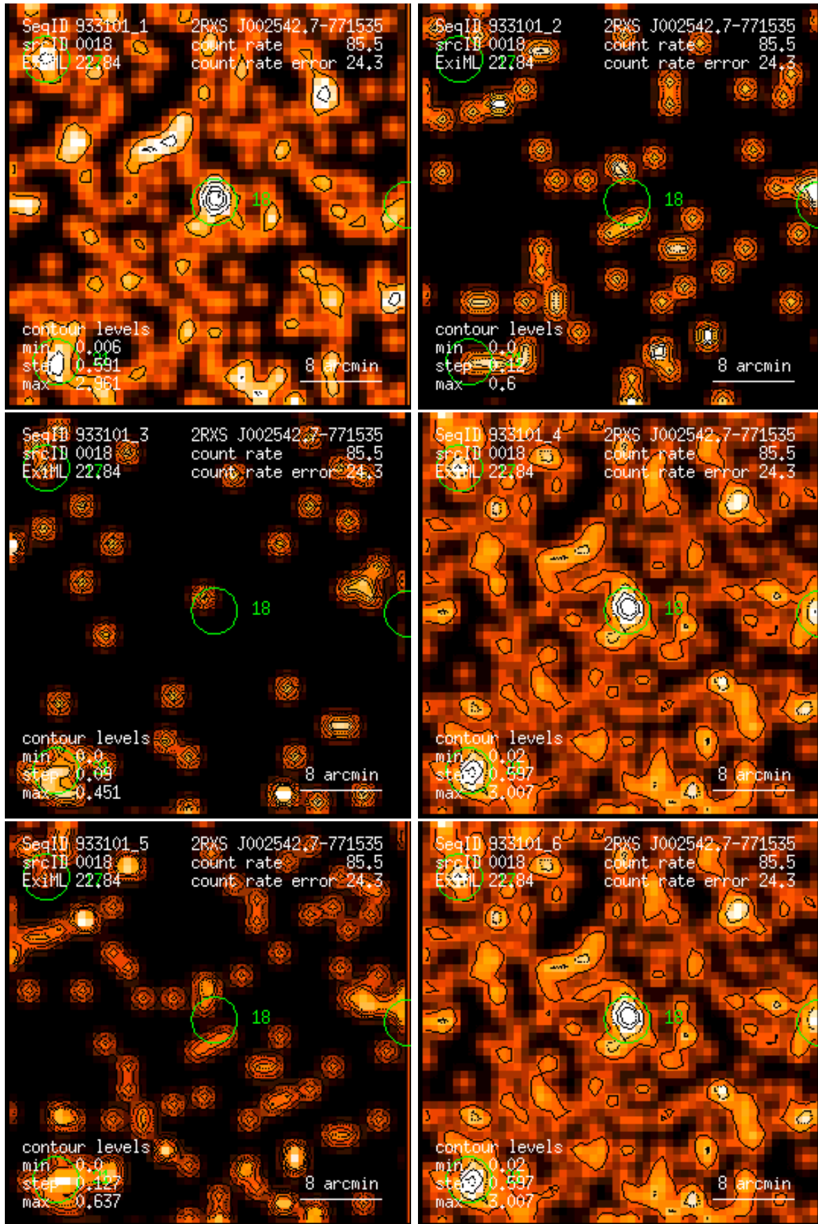
Figure 18: RASS 933101: detection 0018: band rate images, Gaussian filter: (1) PSPC channels 11 – 41, (2) 52 – 90, (3) 91 – 201, (4) 11 – 235, (5) 52 – 201, (6) 11 – 201. Broad band rates in counts/ks. Band rate contour levels in counts/ks/arcmin 2 .
