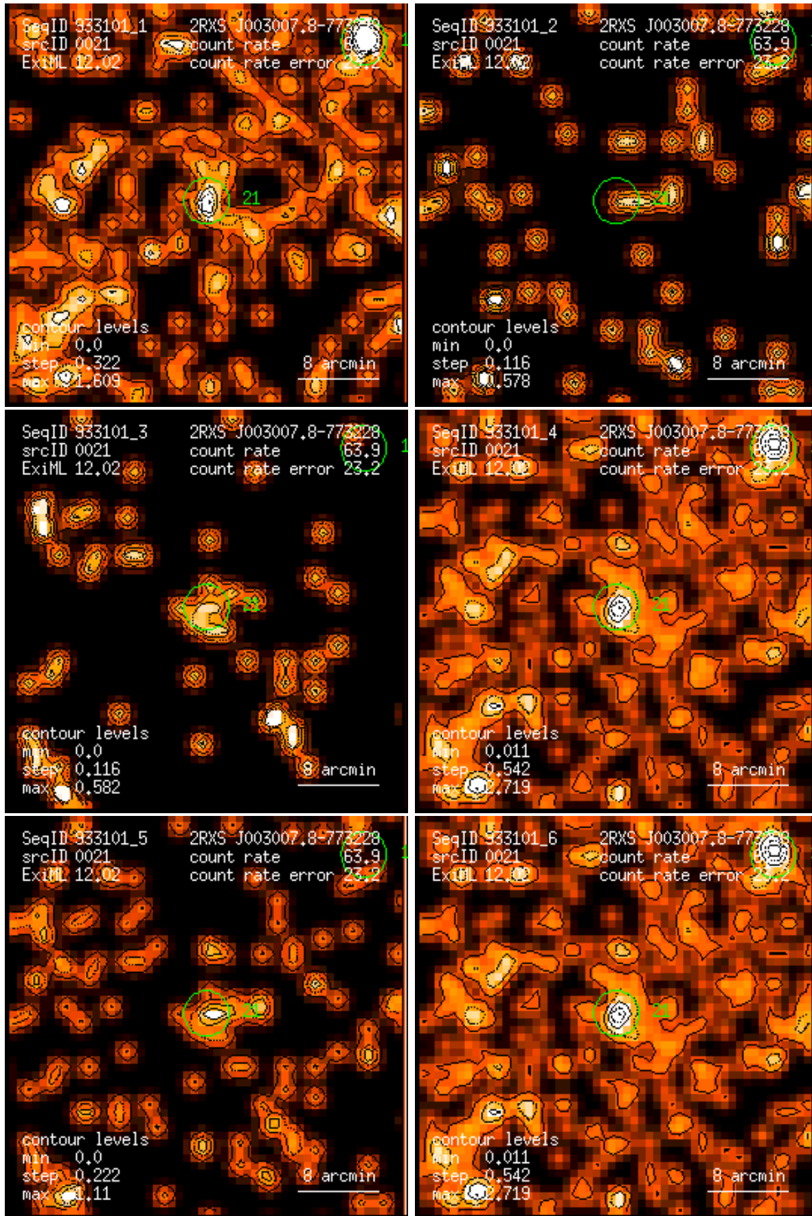
Figure 21: RASS 933101: detection 0021: band rate images, Gaussian filter: (1) PSPC channels 11 – 41, (2) 52 – 90, (3) 91 – 201, (4) 11 – 235, (5) 52 – 201, (6) 11 – 201. Broad band rates in counts/ks. Band rate contour levels in counts/ks/arcmin 2 .
