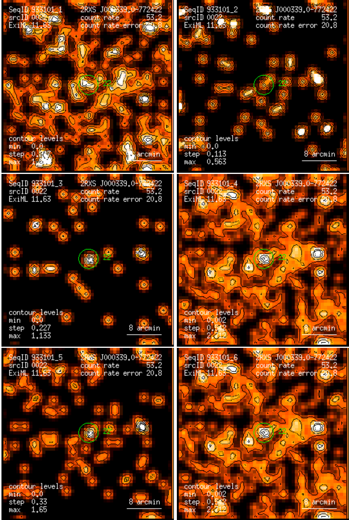
Figure 22: RASS 933101: detection 0022: band rate images, Gaussian filter: (1) PSPC channels 11 – 41, (2) 52 – 90, (3) 91 – 201, (4) 11 – 235, (5) 52 – 201, (6) 11 – 201. Broad band rates in counts/ks. Band rate contour levels in counts/ks/arcmin 2 .
