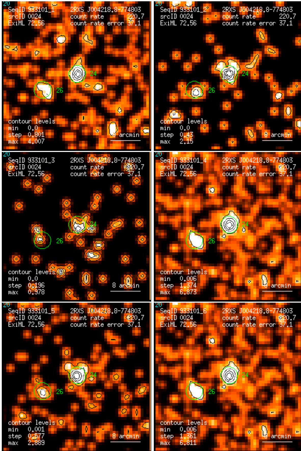
Figure 24: RASS 933101: detection 0024: band rate images, Gaussian filter: (1) PSPC channels 11 – 41, (2) 52 – 90, (3) 91 – 201, (4) 11 – 235, (5) 52 – 201, (6) 11 – 201. Broad band rates in counts/ks. Band rate contour levels in counts/ks/arcmin 2 .
