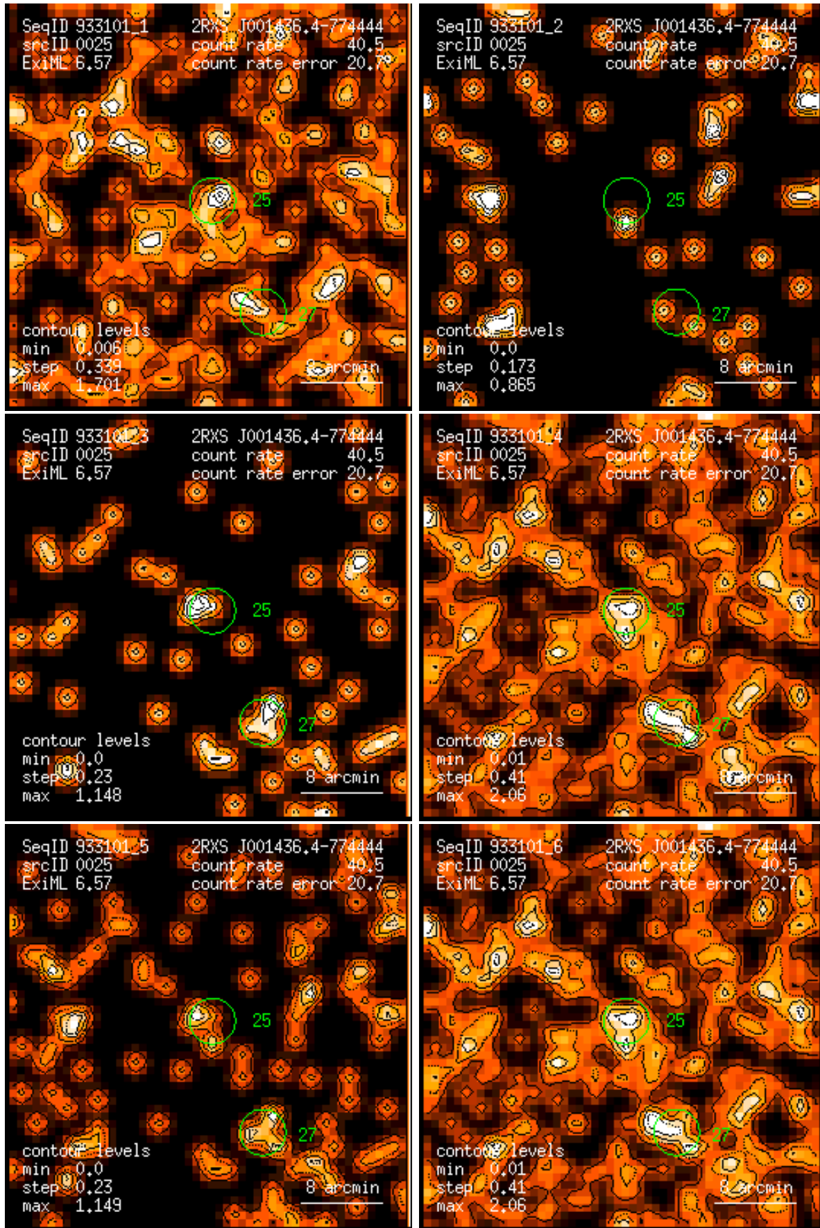
Figure 25: RASS 933101: detection 0025: band rate images, Gaussian filter: (1) PSPC channels 11 – 41, (2) 52 – 90, (3) 91 – 201, (4) 11 – 235, (5) 52 – 201, (6) 11 – 201. Broad band rates in counts/ks. Band rate contour levels in counts/ks/arcmin 2 .
