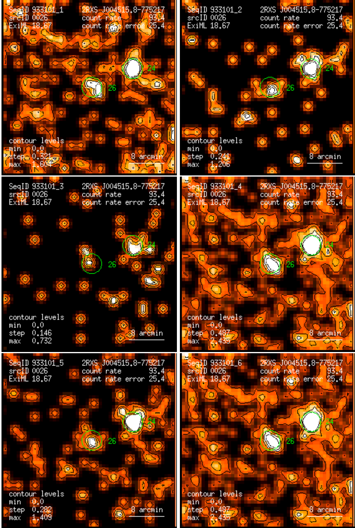
Figure 26: RASS 933101: detection 0026: band rate images, Gaussian filter: (1) PSPC channels 11 – 41, (2) 52 – 90, (3) 91 – 201, (4) 11 – 235, (5) 52 – 201, (6) 11 – 201. Broad band rates in counts/ks. Band rate contour levels in counts/ks/arcmin 2 .
