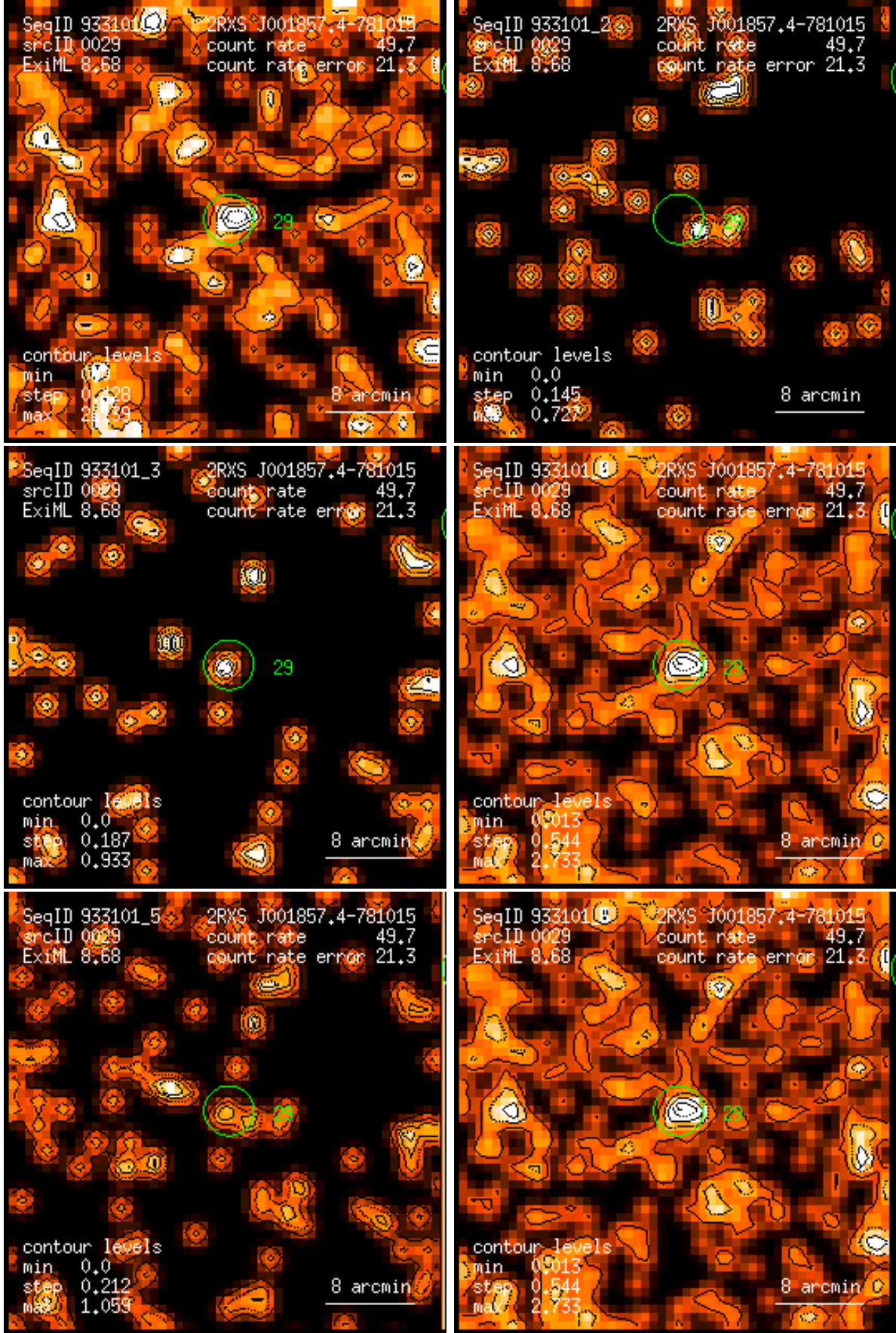
Figure 29: RASS 933101: detection 0029: band rate images, Gaussian filter: (1) PSPC channels 11 – 41, (2) 52 – 90, (3) 91 – 201, (4) 11 – 235, (5) 52 – 201, (6) 11 – 201. Broad band rates in counts/ks. Band rate contour levels in counts/ks/arcmin 2 .
