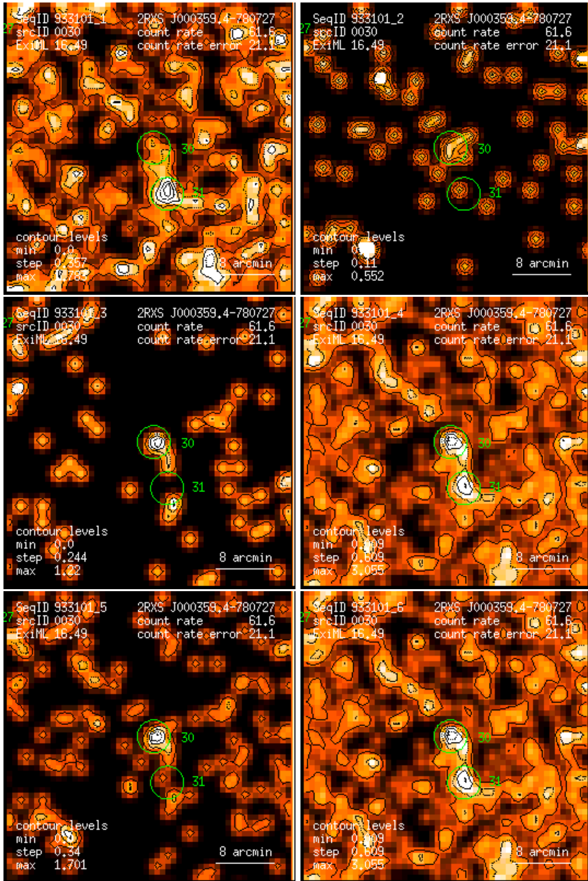
Figure 30: RASS 933101: detection 0030: band rate images, Gaussian filter: (1) PSPC channels 11 – 41, (2) 52 – 90, (3) 91 – 201, (4) 11 – 235, (5) 52 – 201, (6) 11 – 201. Broad band rates in counts/ks. Band rate contour levels in counts/ks/arcmin 2 .
