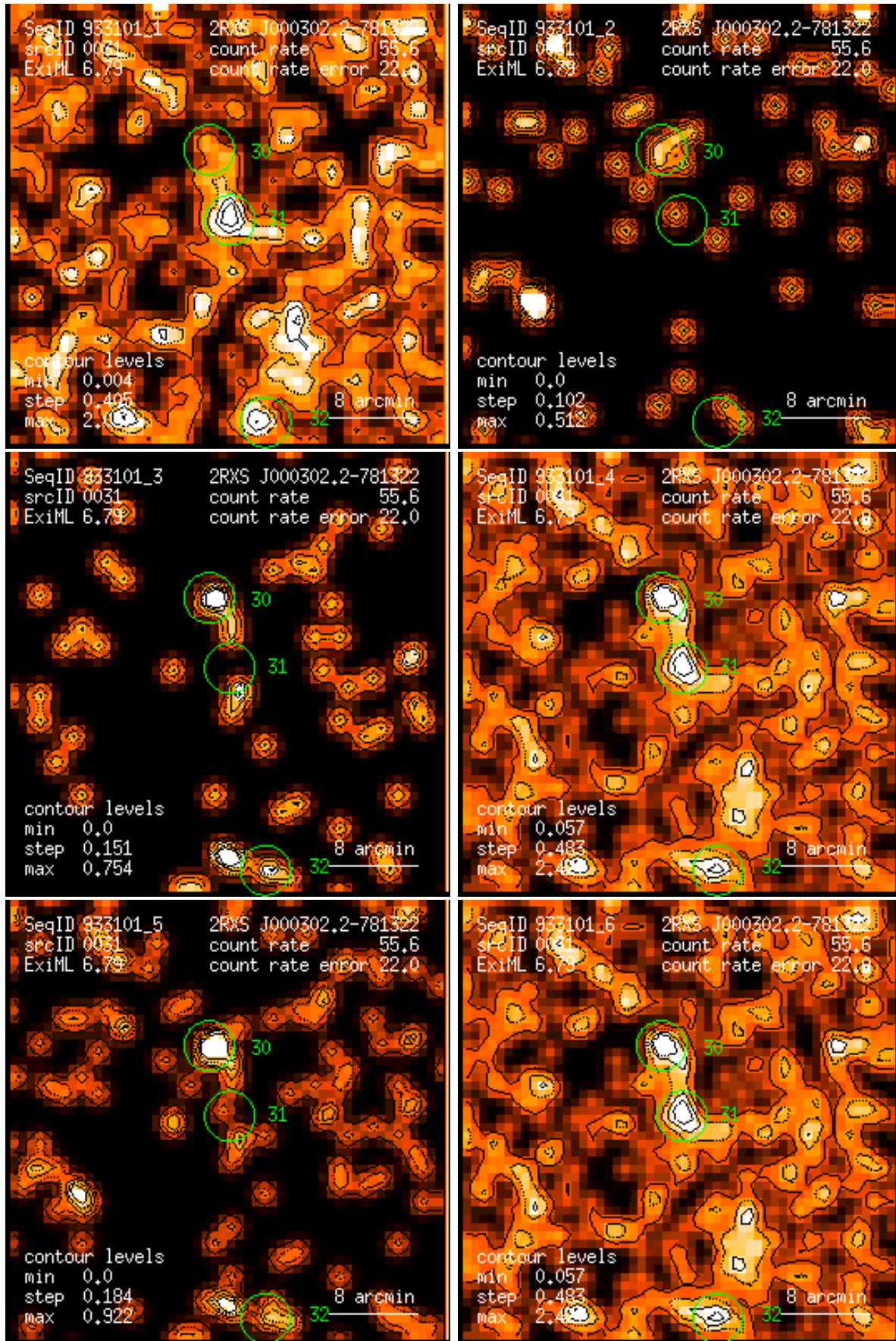
Figure 31: RASS 933101: detection 0031: band rate images, Gaussian filter: (1) PSPC channels 11 – 41, (2) 52 – 90, (3) 91 – 201, (4) 11 – 235, (5) 52 – 201, (6) 11 – 201. Broad band rates in counts/ks. Band rate contour levels in counts/ks/arcmin 2 .
