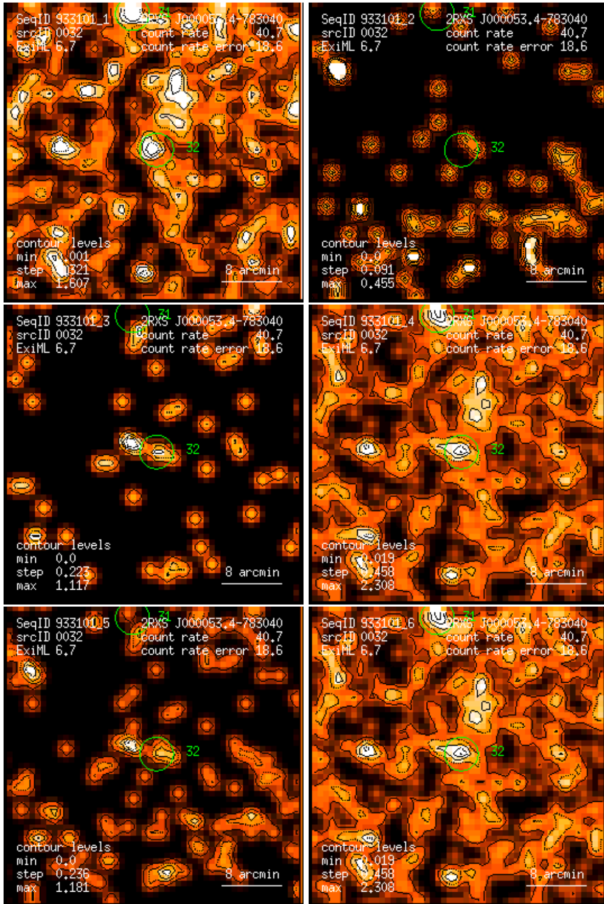
Figure 32: RASS 933101: detection 0032: band rate images, Gaussian filter: (1) PSPC channels 11 – 41, (2) 52 – 90, (3) 91 – 201, (4) 11 – 235, (5) 52 – 201, (6) 11 – 201. Broad band rates in counts/ks. Band rate contour levels in counts/ks/arcmin 2 .
