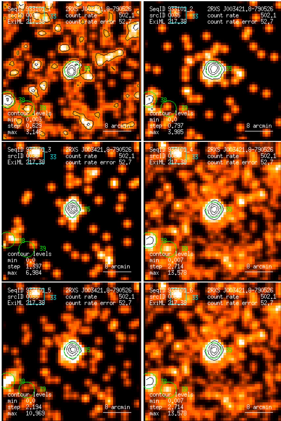
Figure 35: RASS 933101: detection 0035: band rate images, Gaussian filter: (1) PSPC channels 11 – 41, (2) 52 – 90, (3) 91 – 201, (4) 11 – 235, (5) 52 – 201, (6) 11 – 201. Broad band rates in counts/ks. Band rate contour levels in counts/ks/arcmin 2 .
