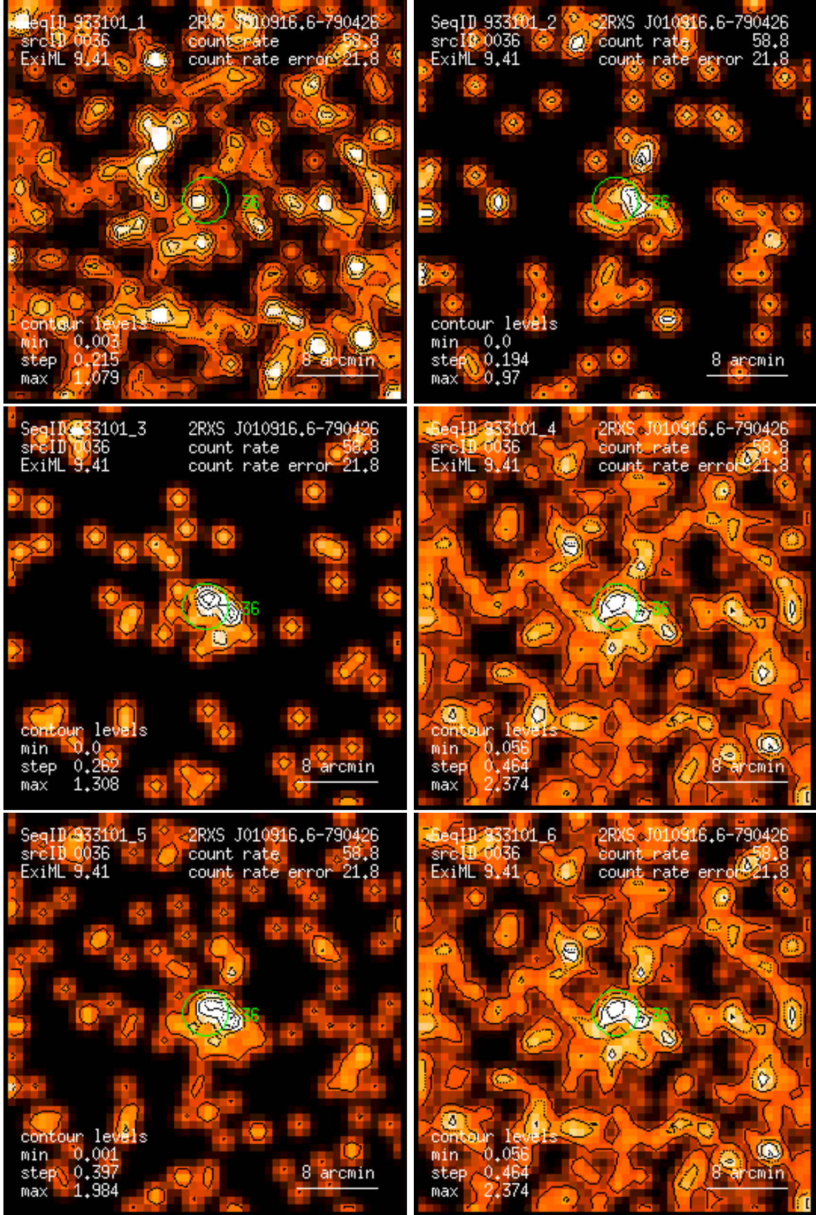
Figure 36: RASS 933101: detection 0036: band rate images, Gaussian filter: (1) PSPC channels 11 – 41, (2) 52 – 90, (3) 91 – 201, (4) 11 – 235, (5) 52 – 201, (6) 11 – 201. Broad band rates in counts/ks. Band rate contour levels in counts/ks/arcmin 2 .
