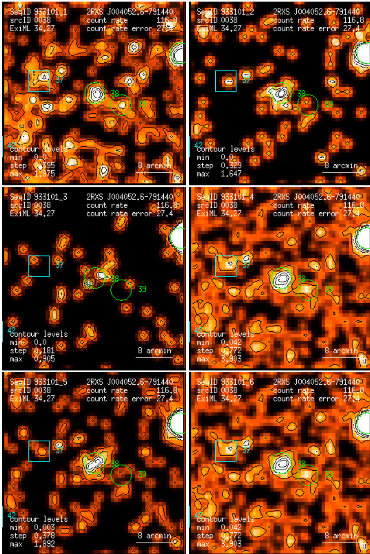
Figure 38: RASS 933101: detection 0038: band rate images, Gaussian filter: (1) PSPC channels 11 – 41, (2) 52 – 90, (3) 91 – 201, (4) 11 – 235, (5) 52 – 201, (6) 11 – 201. Broad band rates in counts/ks. Band rate contour levels in counts/ks/arcmin 2 .
