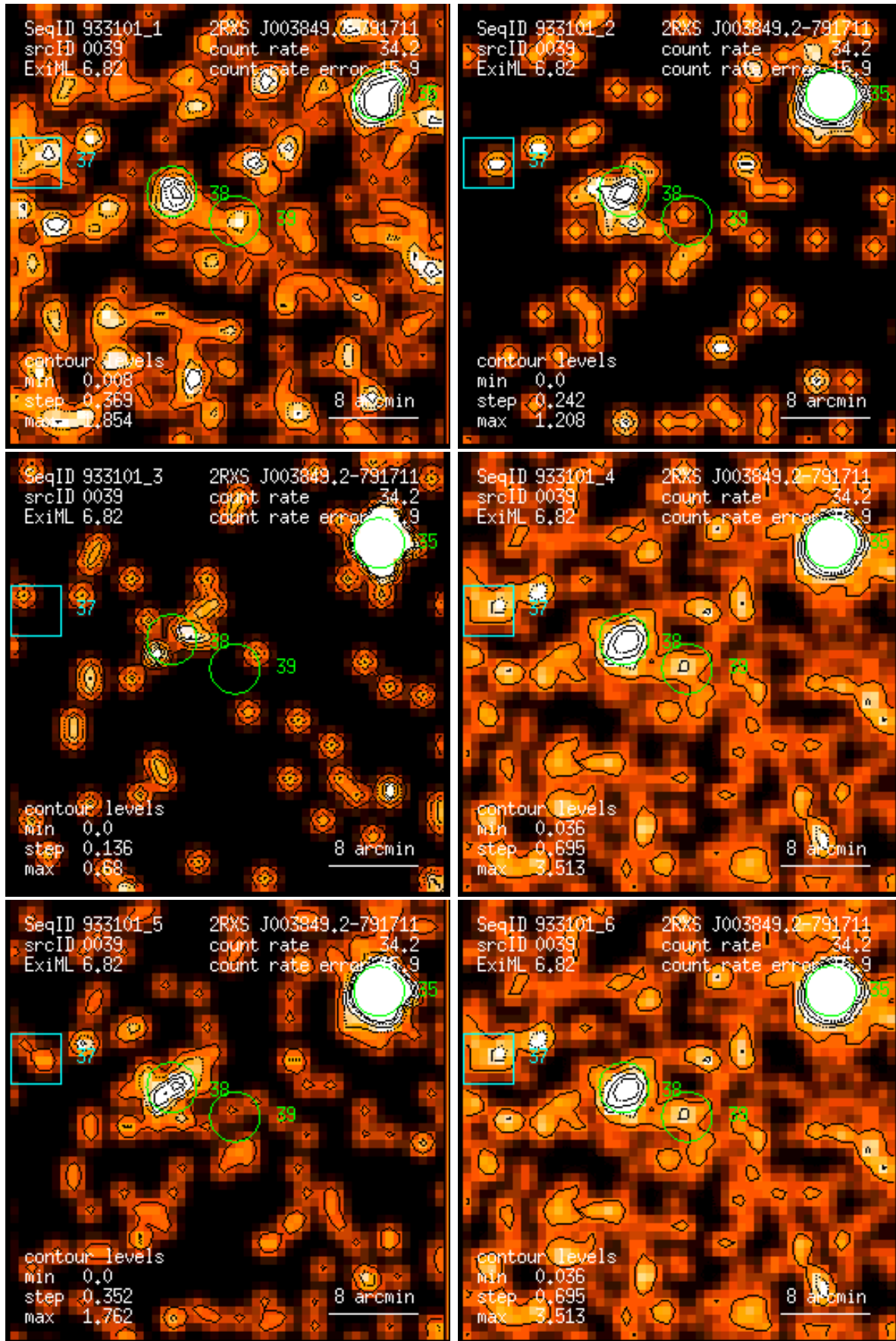
Figure 39: RASS 933101: detection 0039: band rate images, Gaussian filter: (1) PSPC channels 11 – 41, (2) 52 – 90, (3) 91 – 201, (4) 11 – 235, (5) 52 – 201, (6) 11 – 201. Broad band rates in counts/ks. Band rate contour levels in counts/ks/arcmin 2 .
