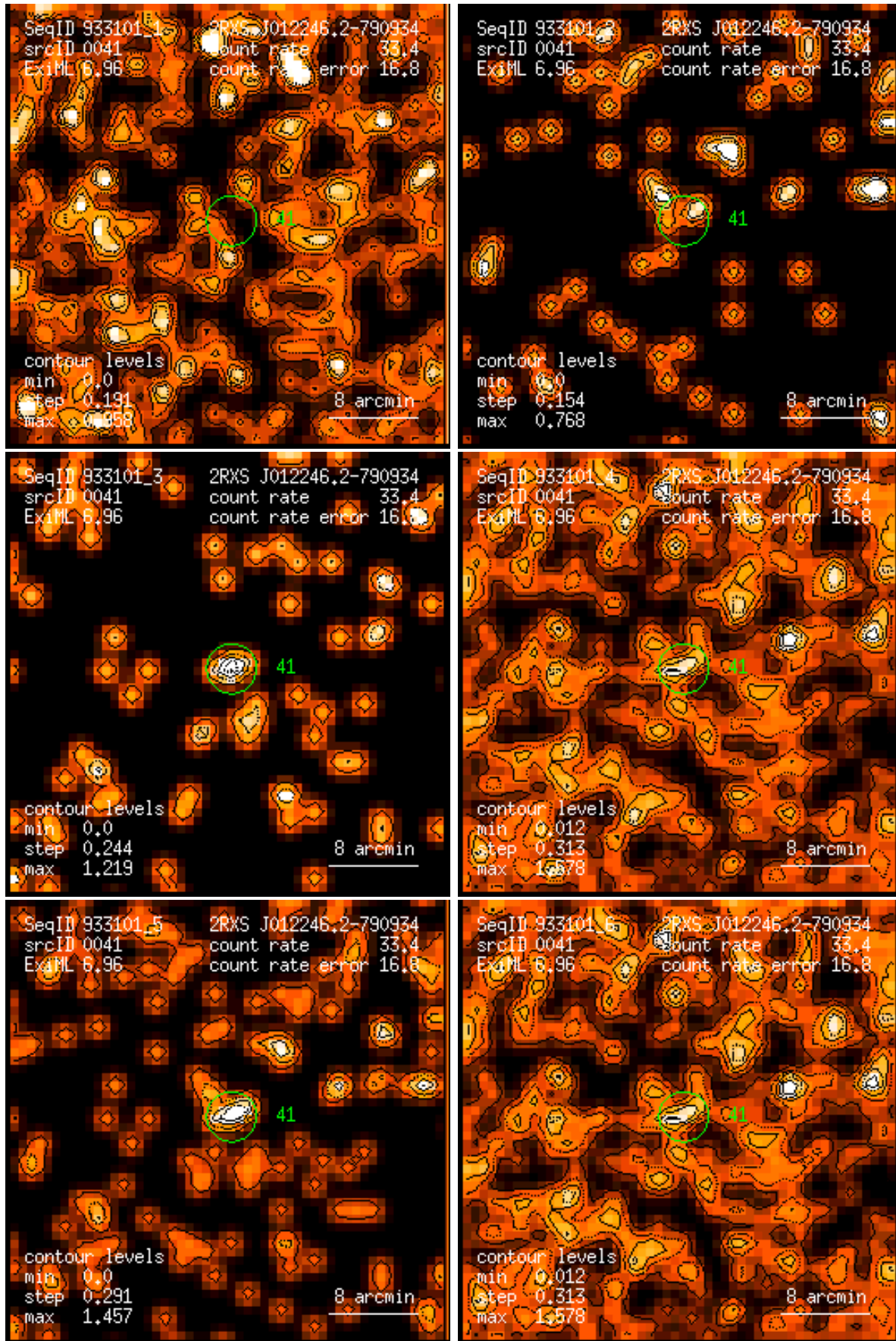
Figure 41: RASS 933101: detection 0041: band rate images, Gaussian filter: (1) PSPC channels 11 – 41, (2) 52 – 90, (3) 91 – 201, (4) 11 – 235, (5) 52 – 201, (6) 11 – 201. Broad band rates in counts/ks. Band rate contour levels in counts/ks/arcmin 2 .
