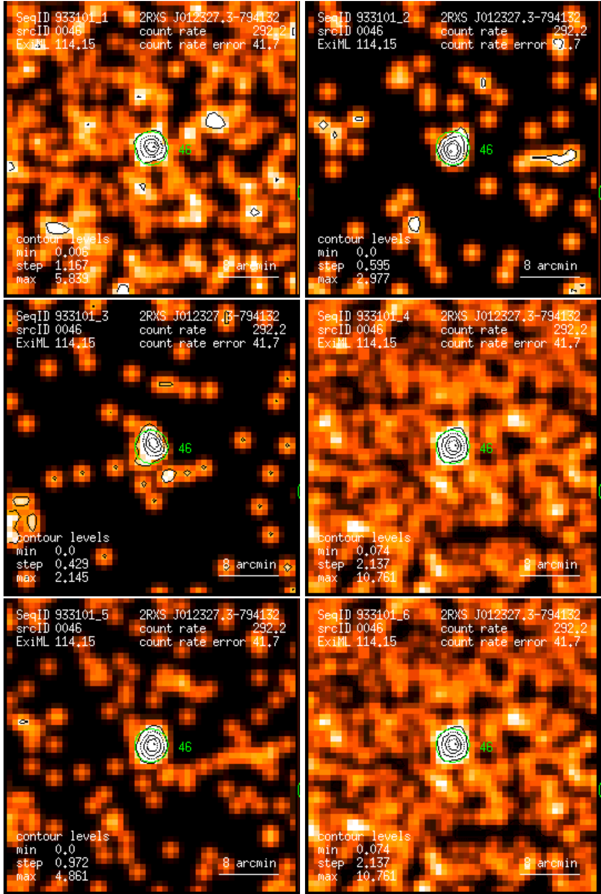
Figure 46: RASS 933101: detection 0046: band rate images, Gaussian filter: (1) PSPC channels 11 – 41, (2) 52 – 90, (3) 91 – 201, (4) 11 – 235, (5) 52 – 201, (6) 11 – 201. Broad band rates in counts/ks. Band rate contour levels in counts/ks/arcmin 2 .
