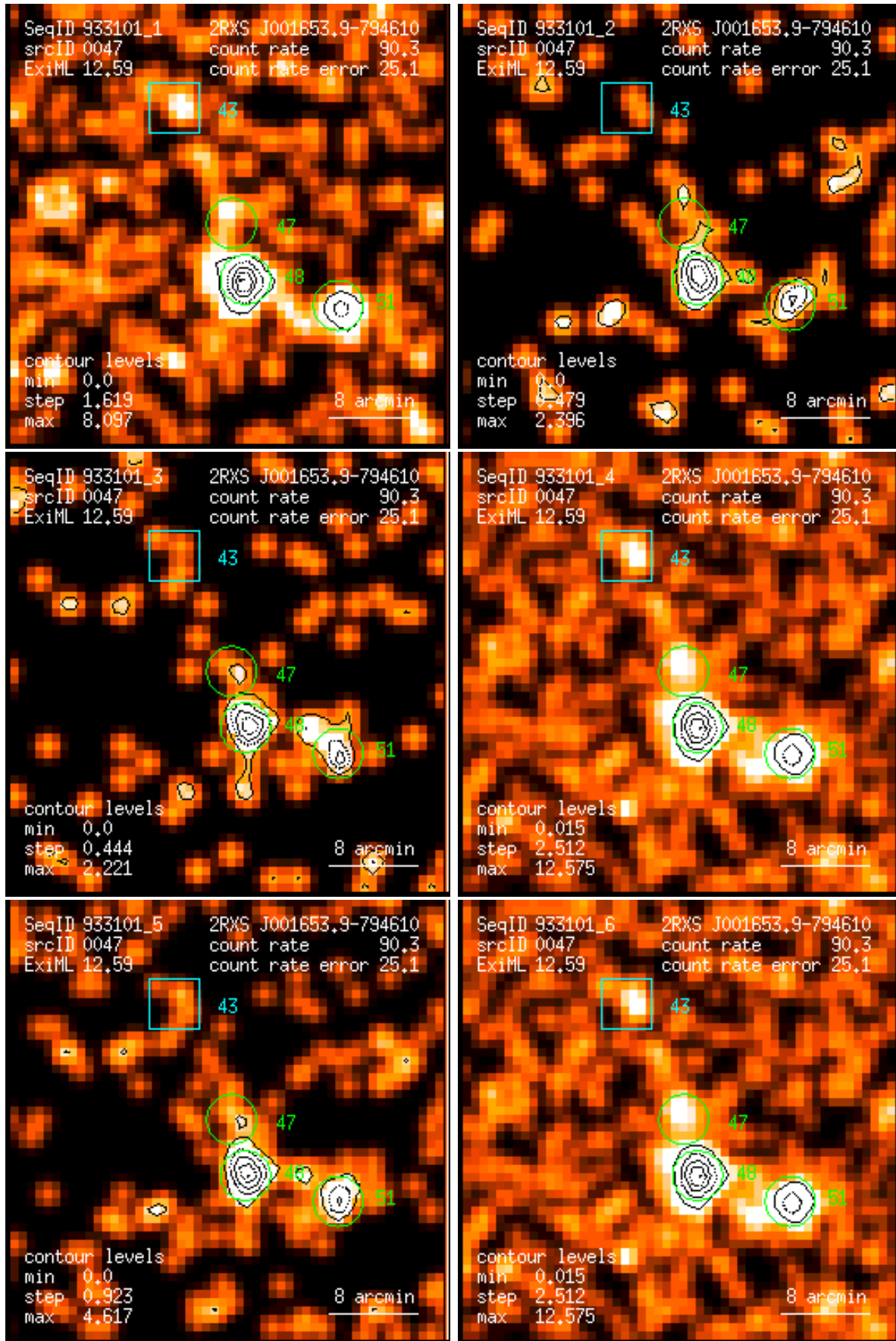
Figure 47: RASS 933101: detection 0047: band rate images, Gaussian filter: (1) PSPC channels 11 – 41, (2) 52 – 90, (3) 91 – 201, (4) 11 – 235, (5) 52 – 201, (6) 11 – 201. Broad band rates in counts/ks. Band rate contour levels in counts/ks/arcmin 2 .
