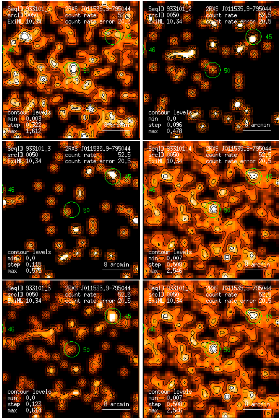
Figure 50: RASS 933101: detection 0050: band rate images, Gaussian filter: (1) PSPC channels 11 – 41, (2) 52 – 90, (3) 91 – 201, (4) 11 – 235, (5) 52 – 201, (6) 11 – 201. Broad band rates in counts/ks. Band rate contour levels in counts/ks/arcmin 2 .
