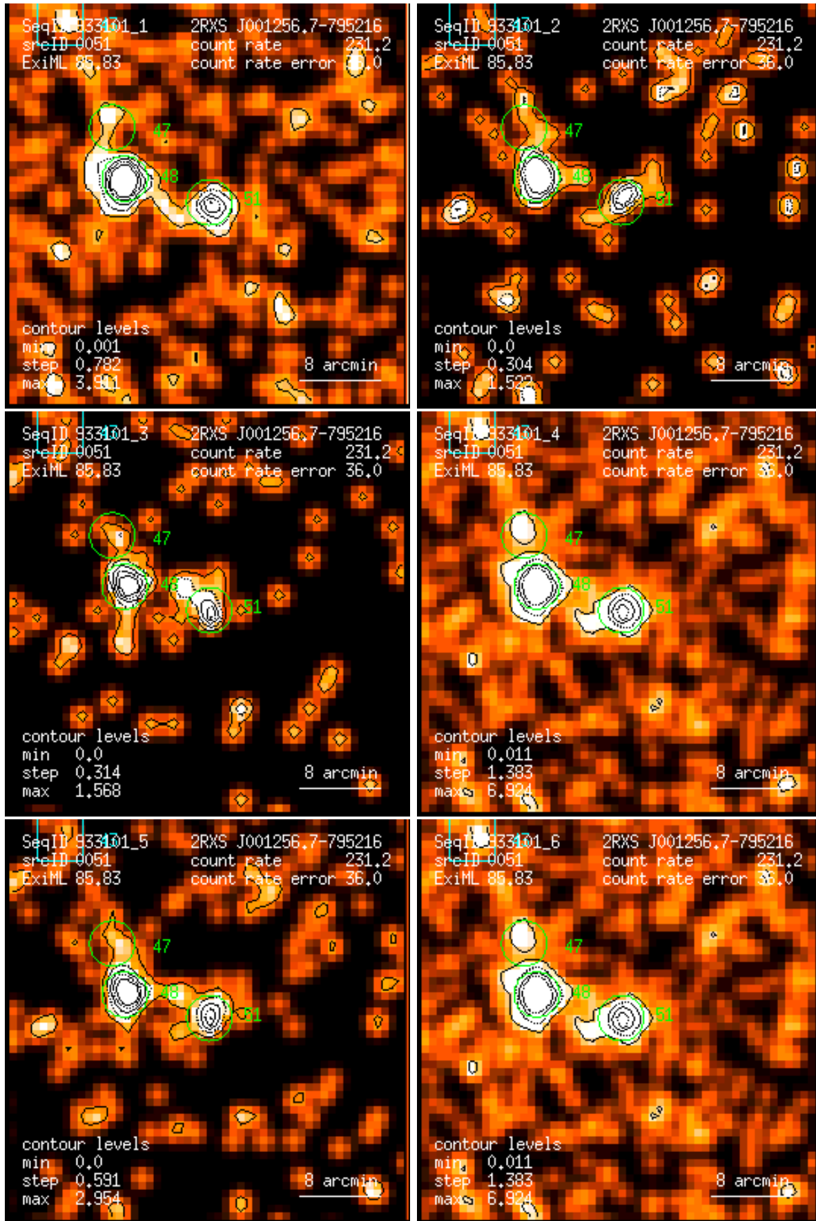
Figure 51: RASS 933101: detection 0051: band rate images, Gaussian filter: (1) PSPC channels 11 – 41, (2) 52 – 90, (3) 91 – 201, (4) 11 – 235, (5) 52 – 201, (6) 11 – 201. Broad band rates in counts/ks. Band rate contour levels in counts/ks/arcmin 2 .
