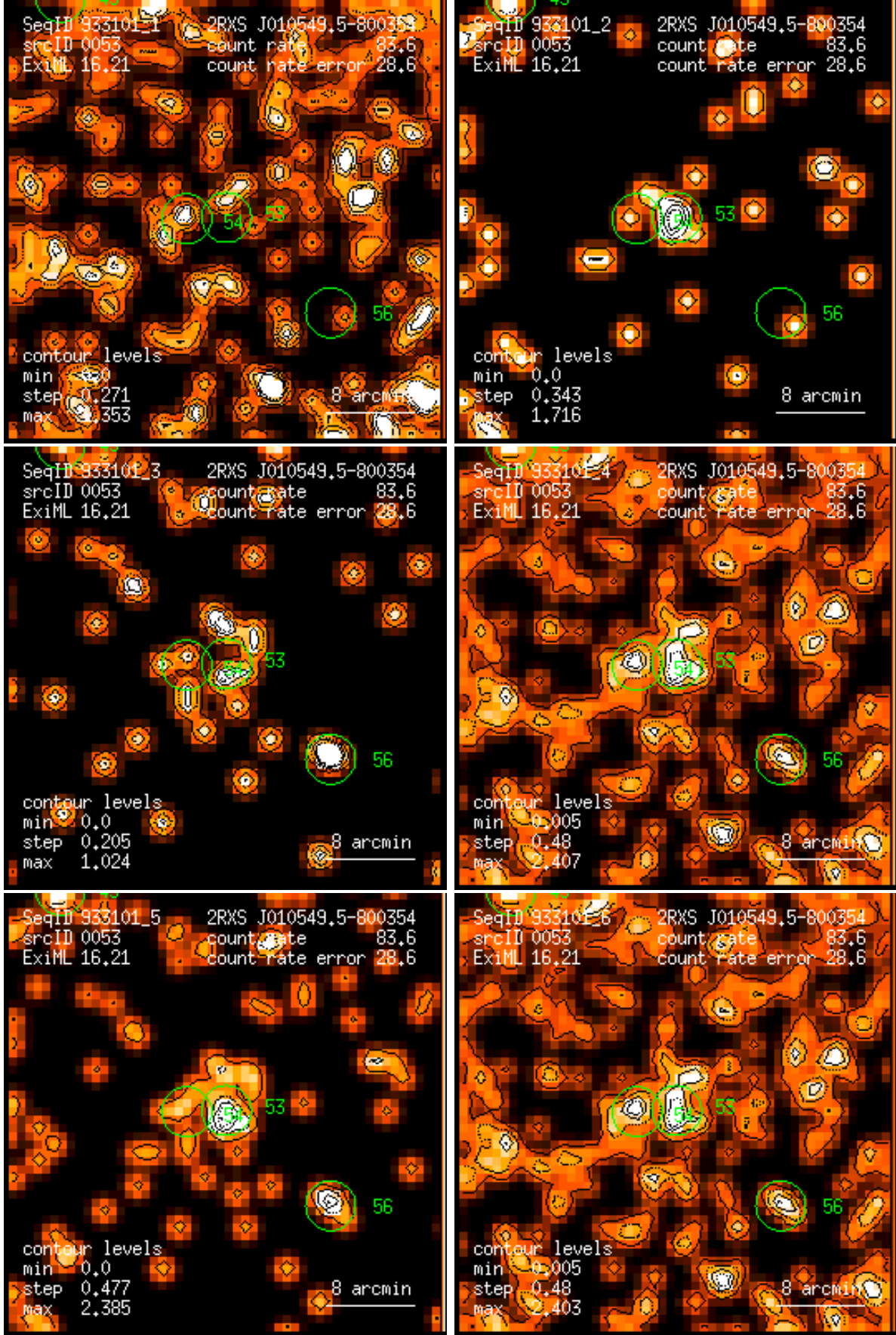
Figure 53: RASS 933101: detection 0053: band rate images, Gaussian filter: (1) PSPC channels 11 – 41, (2) 52 – 90, (3) 91 – 201, (4) 11 – 235, (5) 52 – 201, (6) 11 – 201. Broad band rates in counts/ks. Band rate contour levels in counts/ks/arcmin 2 .
