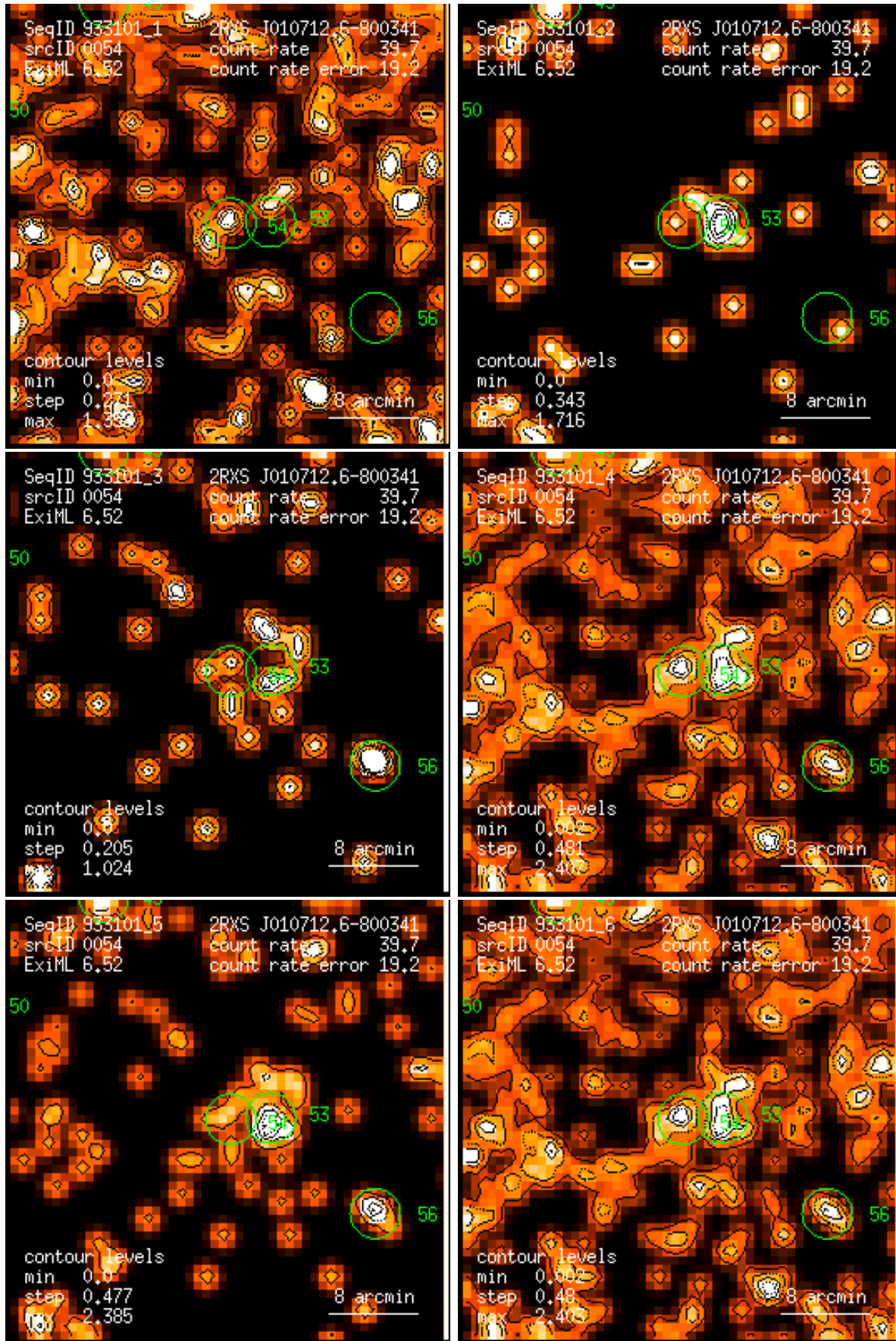
Figure 54: RASS 933101: detection 0054: band rate images, Gaussian filter: (1) PSPC channels 11 – 41, (2) 52 – 90, (3) 91 – 201, (4) 11 – 235, (5) 52 – 201, (6) 11 – 201. Broad band rates in counts/ks. Band rate contour levels in counts/ks/arcmin 2 .
