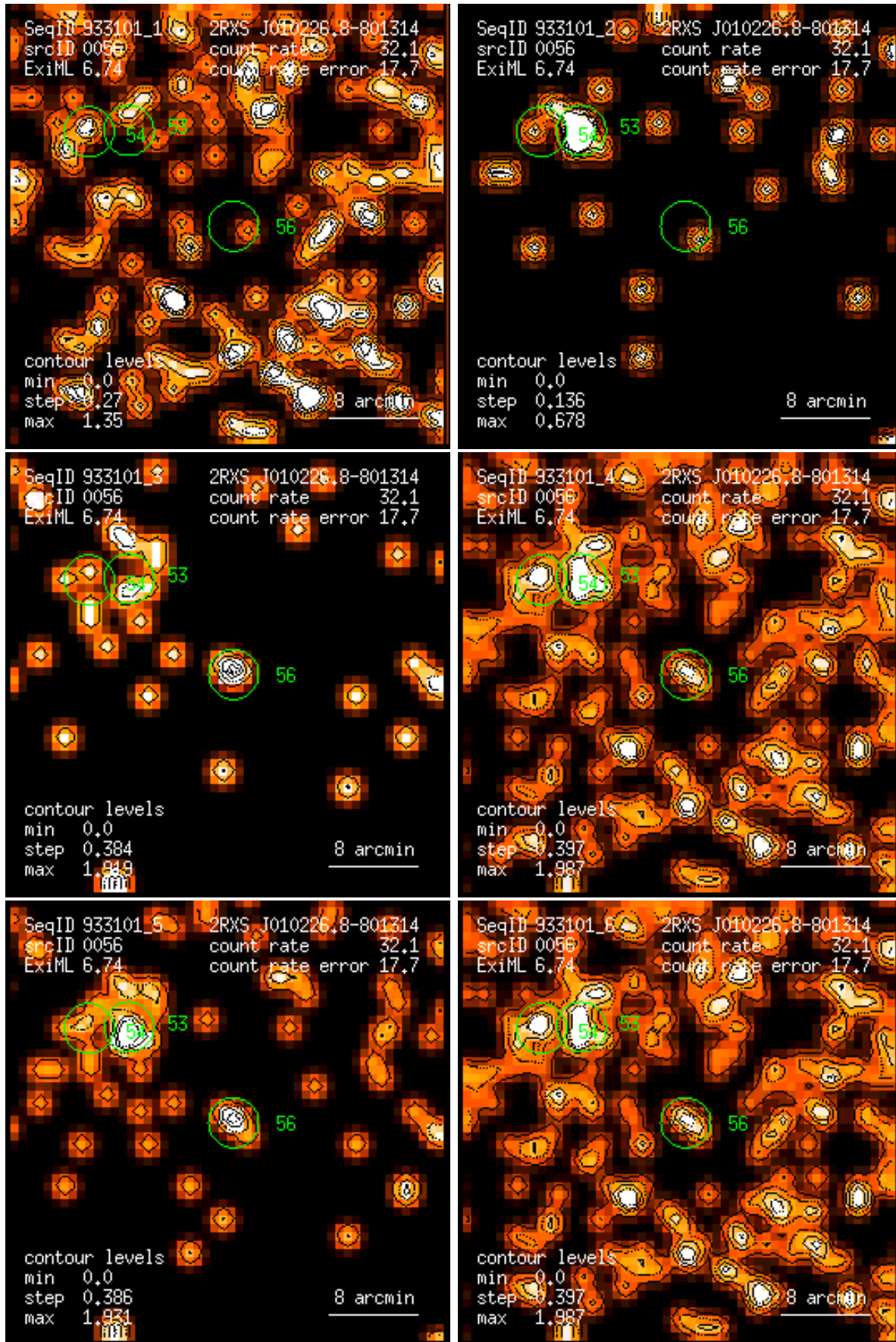
Figure 56: RASS 933101: detection 0056: band rate images, Gaussian filter: (1) PSPC channels 11 – 41, (2) 52 – 90, (3) 91 – 201, (4) 11 – 235, (5) 52 – 201, (6) 11 – 201. Broad band rates in counts/ks. Band rate contour levels in counts/ks/arcmin 2 .
