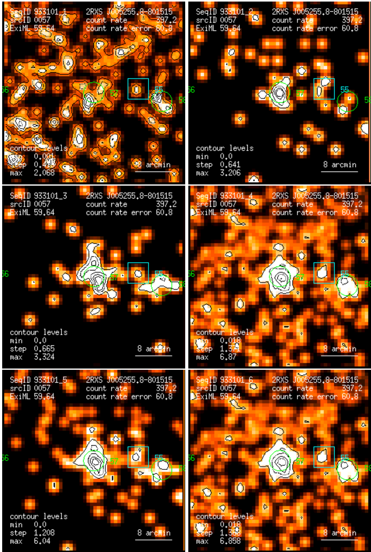
Figure 57: RASS 933101: detection 0057: band rate images, Gaussian filter: (1) PSPC channels 11 – 41, (2) 52 – 90, (3) 91 – 201, (4) 11 – 235, (5) 52 – 201, (6) 11 – 201. Broad band rates in counts/ks. Band rate contour levels in counts/ks/arcmin 2 .
