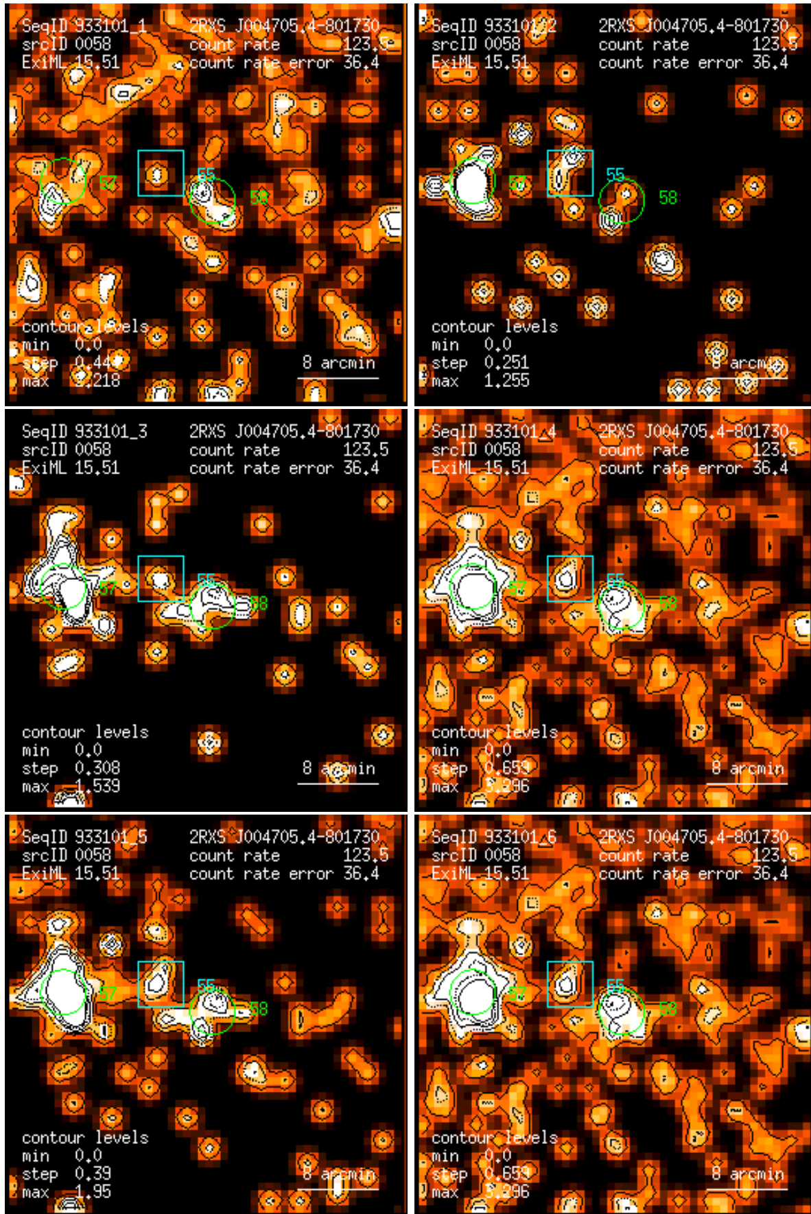
Figure 58: RASS 933101: detection 0058: band rate images, Gaussian filter: (1) PSPC channels 11 – 41, (2) 52 – 90, (3) 91 – 201, (4) 11 – 235, (5) 52 – 201, (6) 11 – 201. Broad band rates in counts/ks. Band rate contour levels in counts/ks/arcmin 2 .
