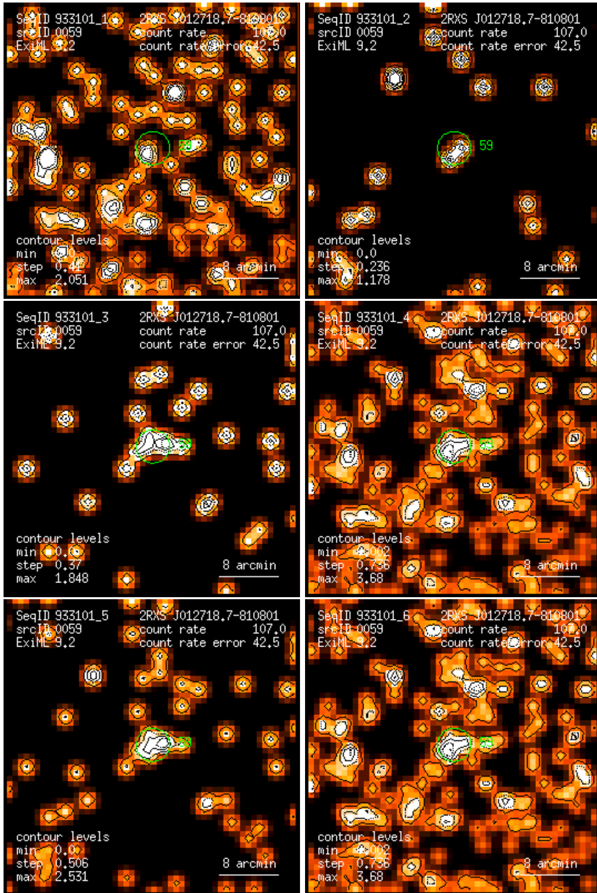
Figure 59: RASS 933101: detection 0059: band rate images, Gaussian filter: (1) PSPC channels 11 – 41, (2) 52 – 90, (3) 91 – 201, (4) 11 – 235, (5) 52 – 201, (6) 11 – 201. Broad band rates in counts/ks. Band rate contour levels in counts/ks/arcmin 2 .
