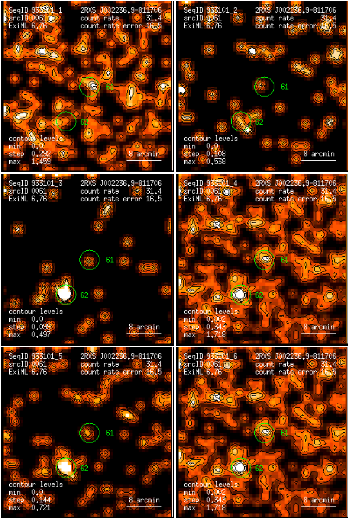
Figure 61: RASS 933101: detection 0061: band rate images, Gaussian filter: (1) PSPC channels 11 – 41, (2) 52 – 90, (3) 91 – 201, (4) 11 – 235, (5) 52 – 201, (6) 11 – 201. Broad band rates in counts/ks. Band rate contour levels in counts/ks/arcmin 2 .
