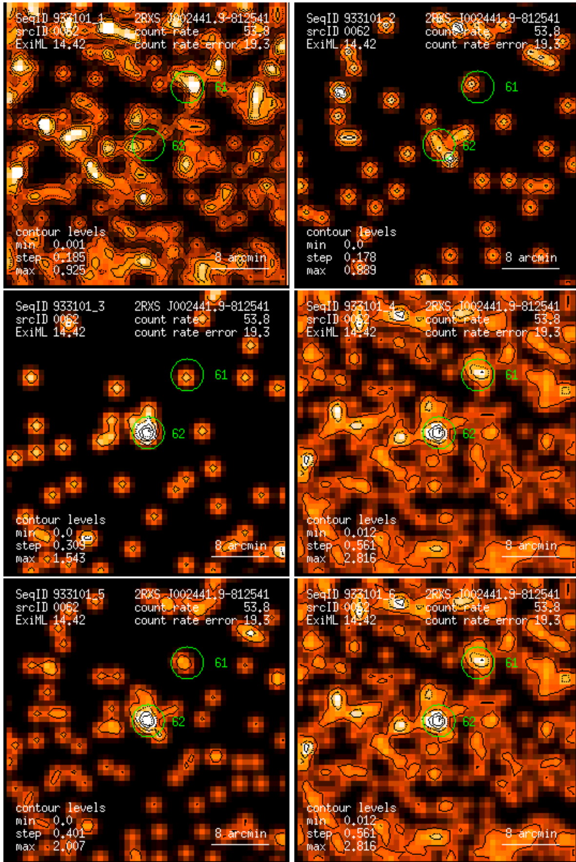
Figure 62: RASS 933101: detection 0062: band rate images, Gaussian filter: (1) PSPC channels 11 – 41, (2) 52 – 90, (3) 91 – 201, (4) 11 – 235, (5) 52 – 201, (6) 11 – 201. Broad band rates in counts/ks. Band rate contour levels in counts/ks/arcmin 2 .
