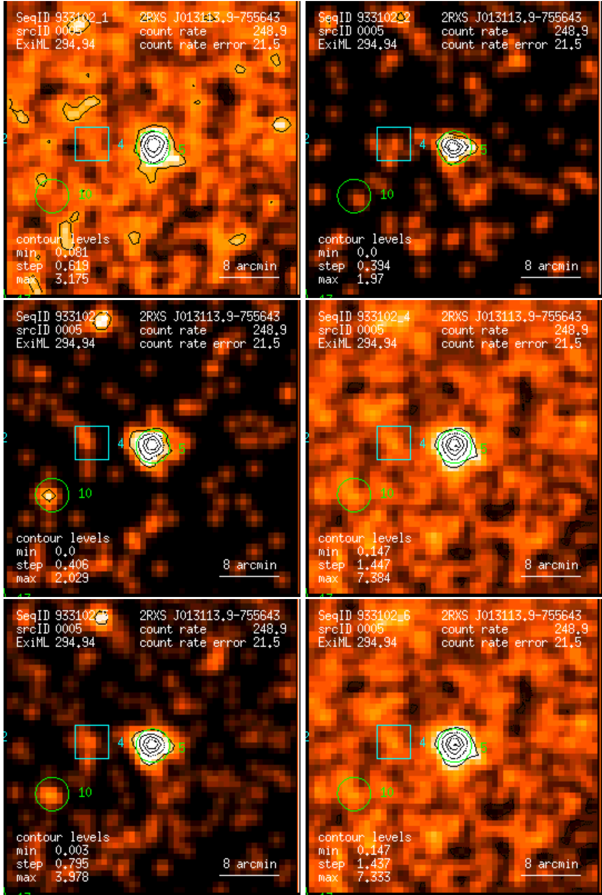
Figure 5: RASS 933102: detection 0005: band rate images, Gaussian filter: (1) PSPC channels 11 – 41, (2) 52 – 90, (3) 91 – 201, (4) 11 – 235, (5) 52 – 201, (6) 11 – 201. Broad band rates in counts/ks. Band rate contour levels in counts/ks/arcmin 2 .
