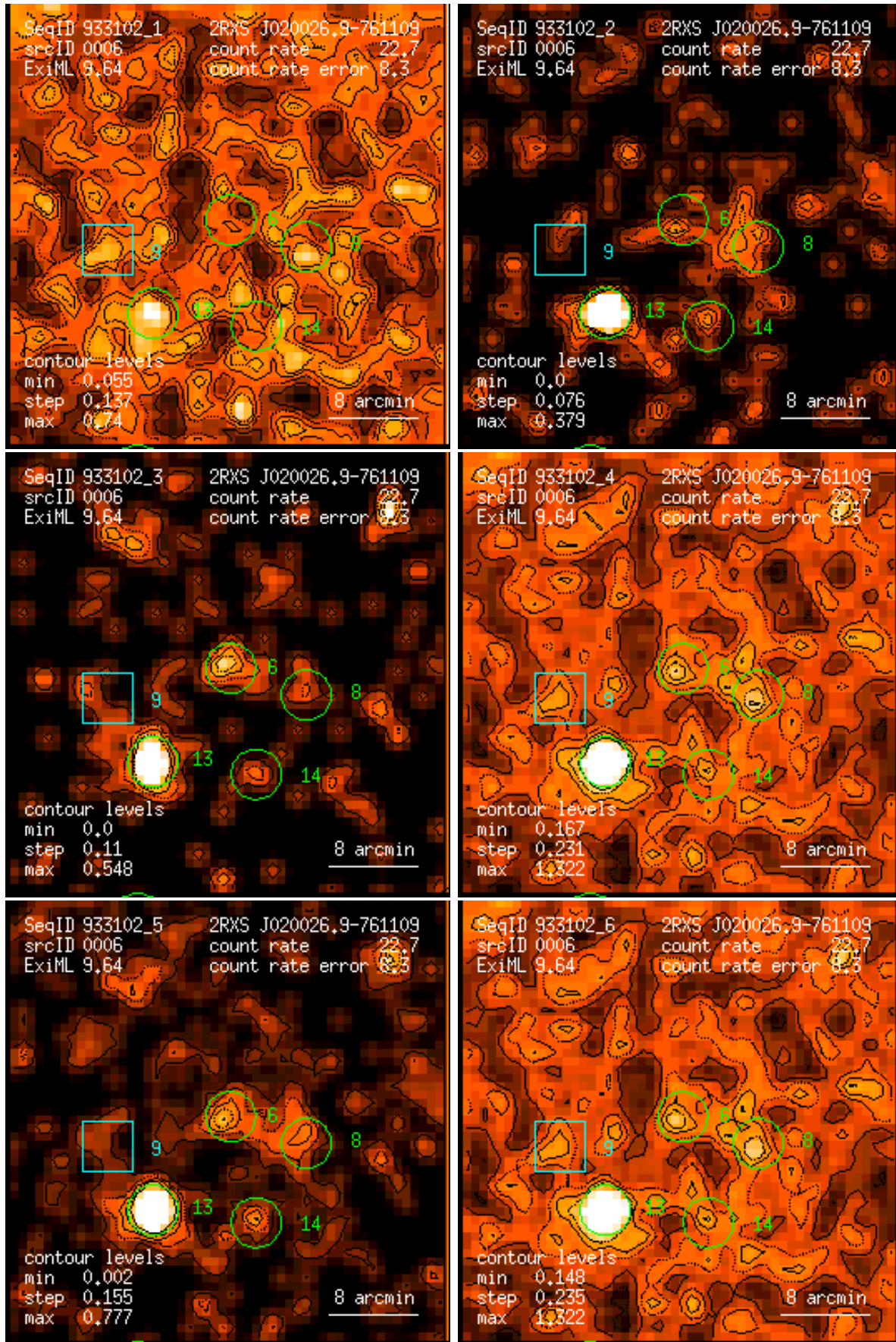
Figure 6: RASS 933102: detection 0006: band rate images, Gaussian filter: (1) PSPC channels 11 – 41, (2) 52 – 90, (3) 91 – 201, (4) 11 – 235, (5) 52 – 201, (6) 11 – 201. Broad band rates in counts/ks. Band rate contour levels in counts/ks/arcmin 2 .
