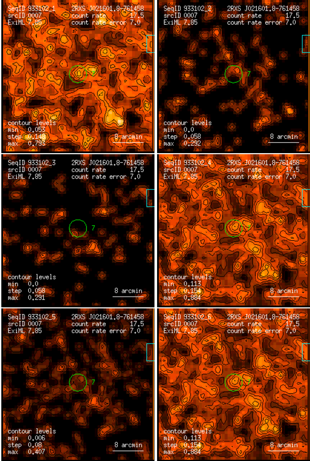
Figure 7: RASS 933102: detection 0007: band rate images, Gaussian filter: (1) PSPC channels 11 – 41, (2) 52 – 90, (3) 91 – 201, (4) 11 – 235, (5) 52 – 201, (6) 11 – 201. Broad band rates in counts/ks. Band rate contour levels in counts/ks/arcmin 2 .
