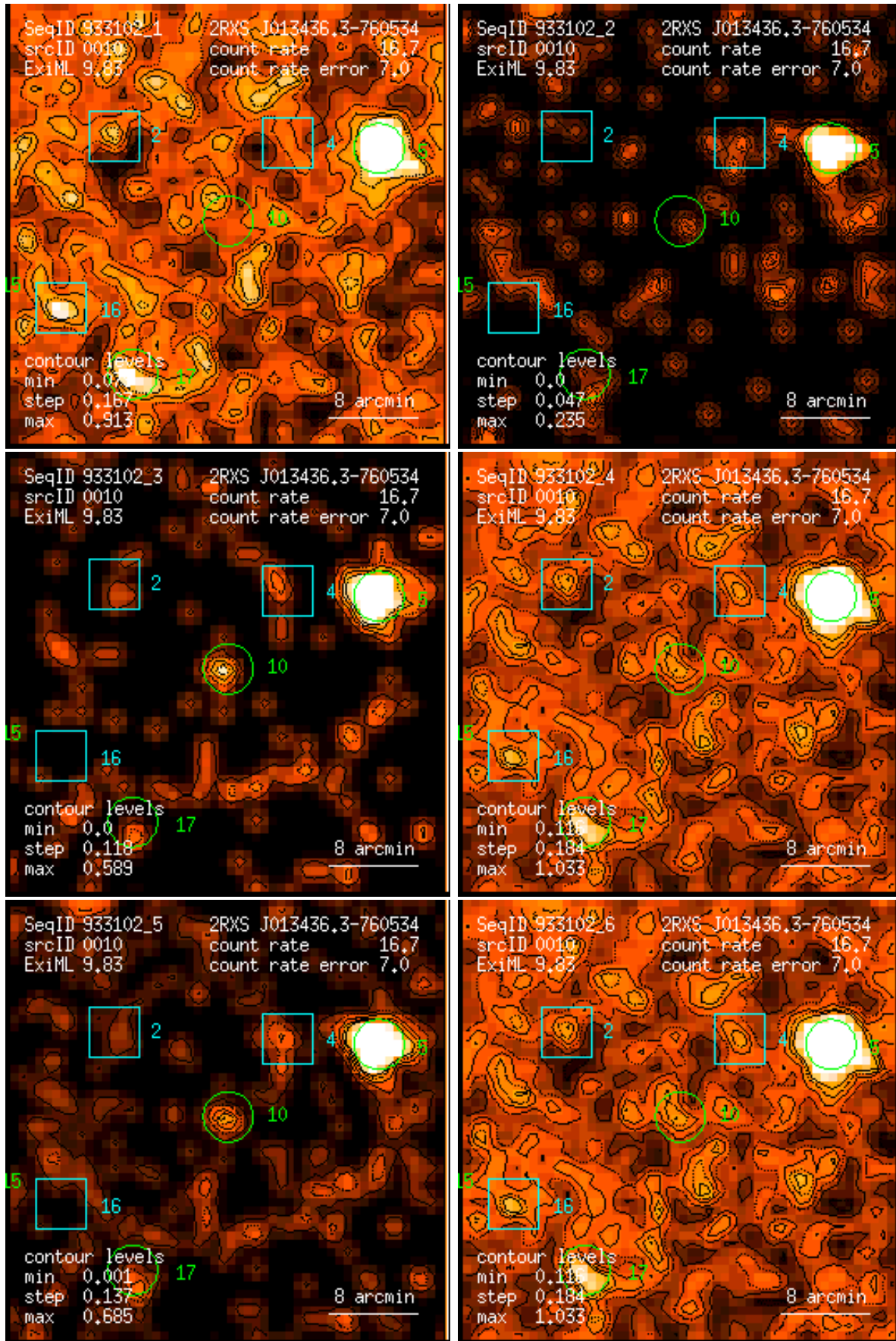
Figure 10: RASS 933102: detection 0010: band rate images, Gaussian filter: (1) PSPC channels 11 – 41, (2) 52 – 90, (3) 91 – 201, (4) 11 – 235, (5) 52 – 201, (6) 11 – 201. Broad band rates in counts/ks. Band rate contour levels in counts/ks/arcmin 2 .
