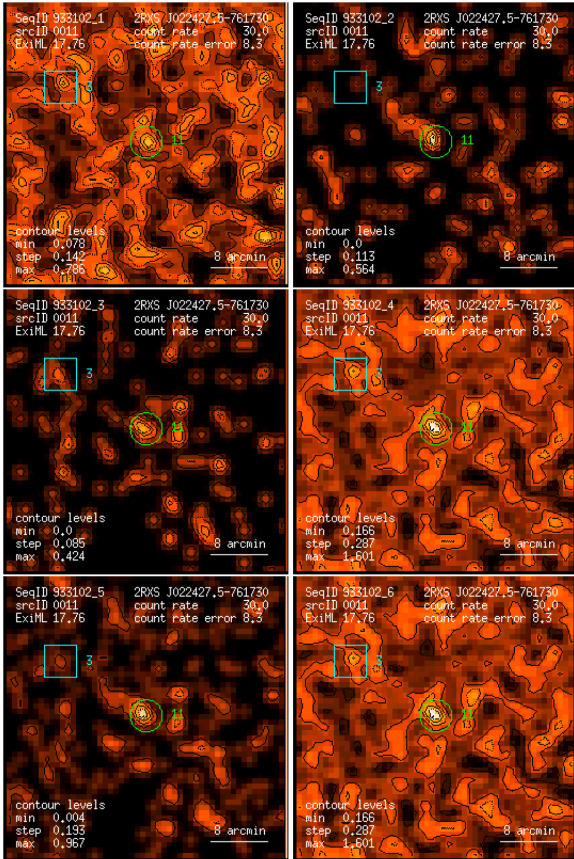
Figure 11: RASS 933102: detection 0011: band rate images, Gaussian filter: (1) PSPC channels 11 – 41, (2) 52 – 90, (3) 91 – 201, (4) 11 – 235, (5) 52 – 201, (6) 11 – 201. Broad band rates in counts/ks. Band rate contour levels in counts/ks/arcmin 2 .
