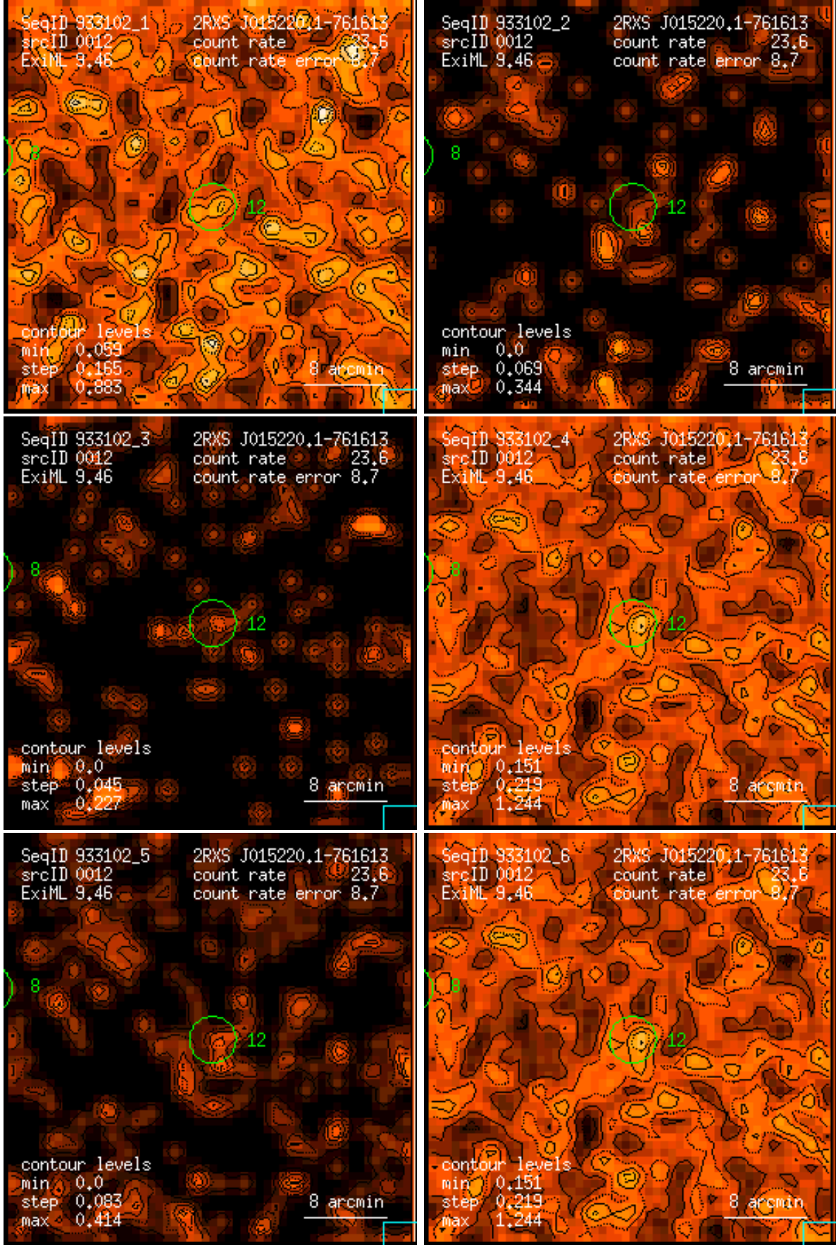
Figure 12: RASS 933102: detection 0012: band rate images, Gaussian filter: (1) PSPC channels 11 – 41, (2) 52 – 90, (3) 91 – 201, (4) 11 – 235, (5) 52 – 201, (6) 11 – 201. Broad band rates in counts/ks. Band rate contour levels in counts/ks/arcmin 2 .
