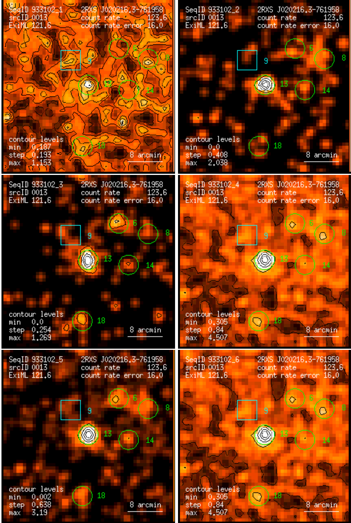
Figure 13: RASS 933102: detection 0013: band rate images, Gaussian filter: (1) PSPC channels 11 – 41, (2) 52 – 90, (3) 91 – 201, (4) 11 – 235, (5) 52 – 201, (6) 11 – 201. Broad band rates in counts/ks. Band rate contour levels in counts/ks/arcmin 2 .
