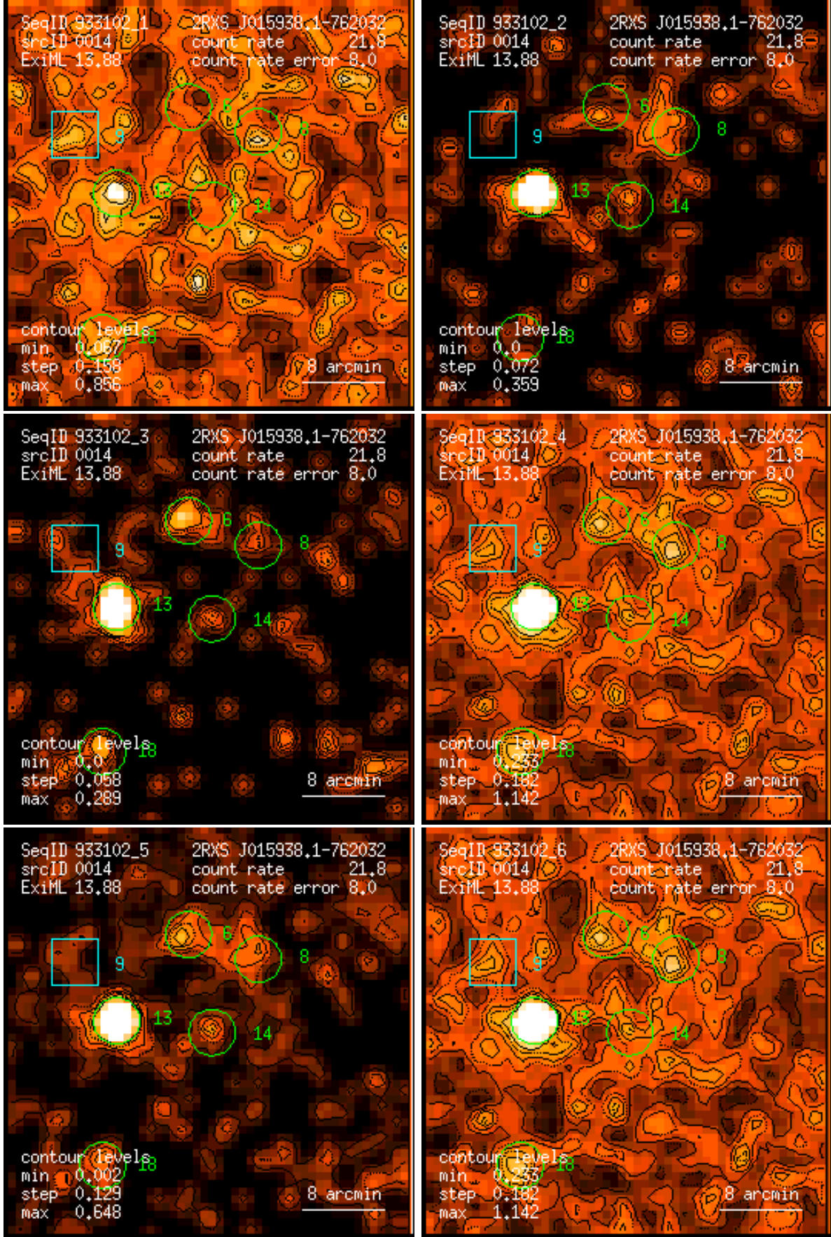
Figure 14: RASS 933102: detection 0014: band rate images, Gaussian filter: (1) PSPC channels 11 – 41, (2) 52 – 90, (3) 91 – 201, (4) 11 – 235, (5) 52 – 201, (6) 11 – 201. Broad band rates in counts/ks. Band rate contour levels in counts/ks/arcmin 2 .
