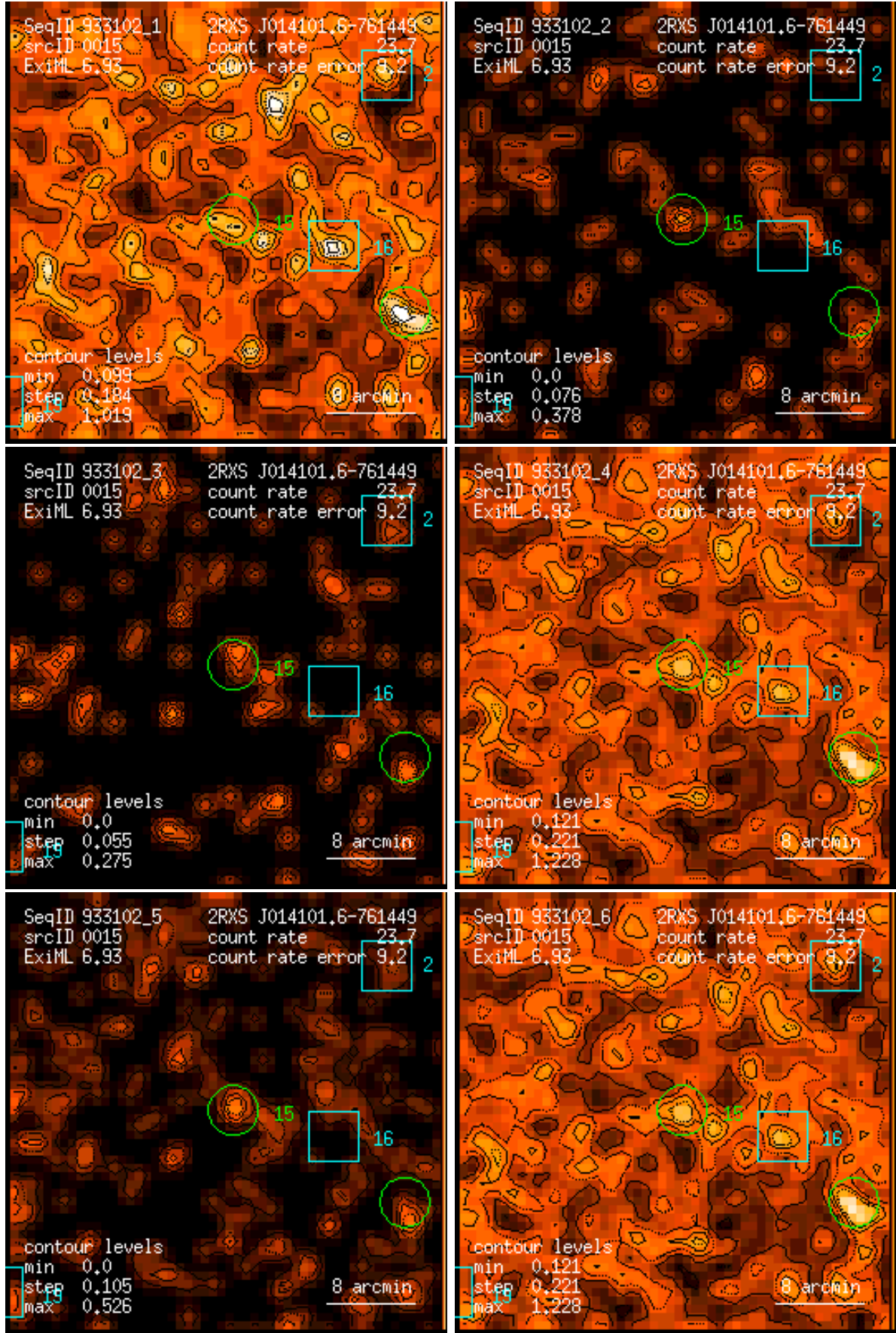
Figure 15: RASS 933102: detection 0015: band rate images, Gaussian filter: (1) PSPC channels 11 – 41, (2) 52 – 90, (3) 91 – 201, (4) 11 – 235, (5) 52 – 201, (6) 11 – 201. Broad band rates in counts/ks. Band rate contour levels in counts/ks/arcmin 2 .
