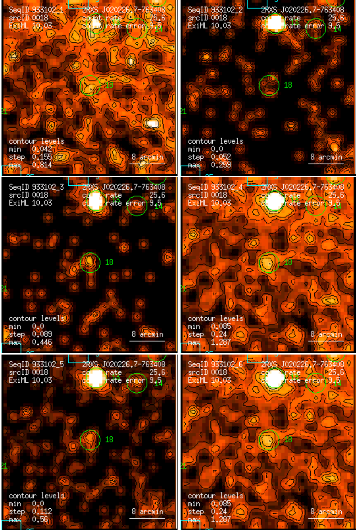
Figure 18: RASS 933102: detection 0018: band rate images, Gaussian filter: (1) PSPC channels 11 – 41, (2) 52 – 90, (3) 91 – 201, (4) 11 – 235, (5) 52 – 201, (6) 11 – 201. Broad band rates in counts/ks. Band rate contour levels in counts/ks/arcmin 2 .
