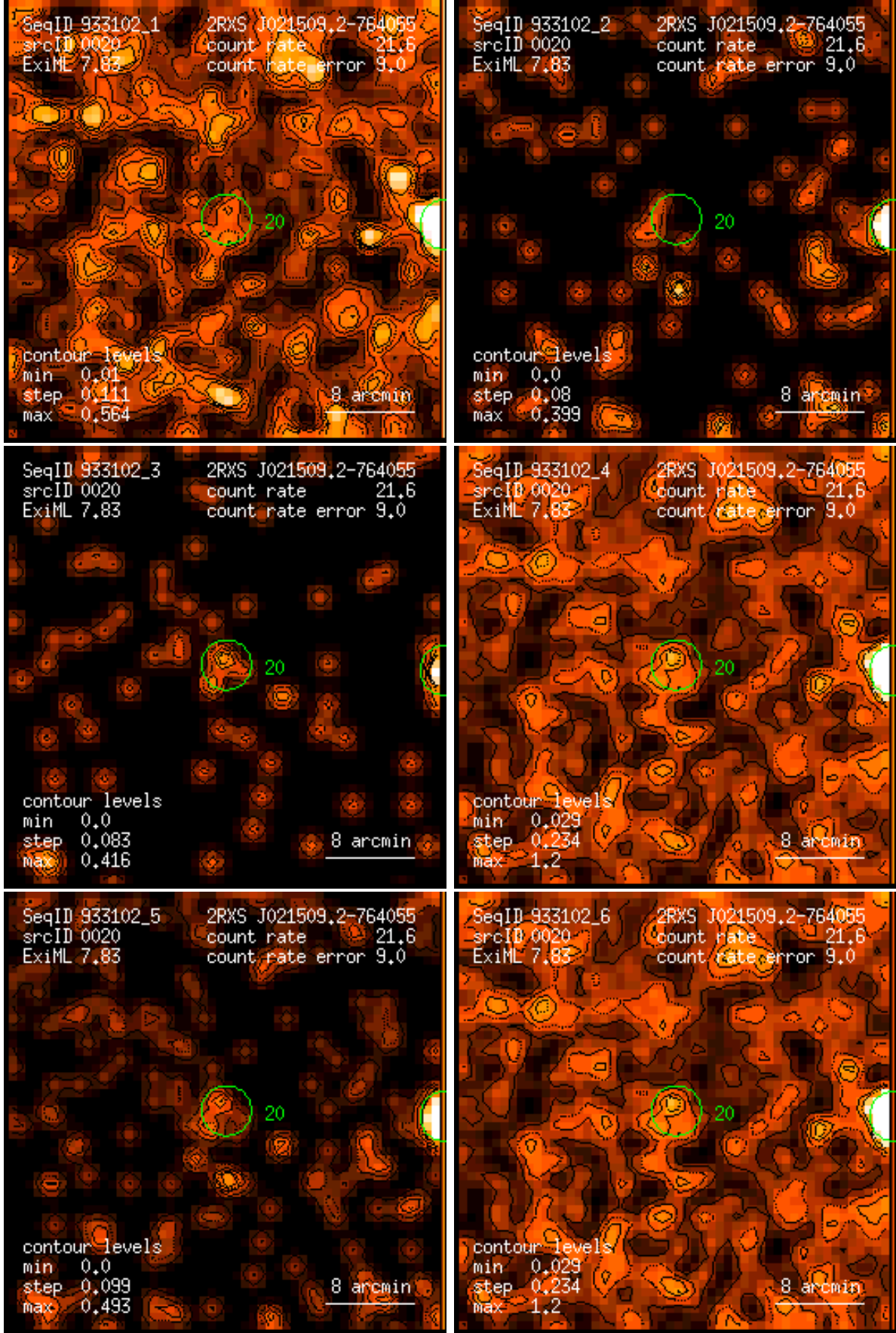
Figure 20: RASS 933102: detection 0020: band rate images, Gaussian filter: (1) PSPC channels 11 – 41, (2) 52 – 90, (3) 91 – 201, (4) 11 – 235, (5) 52 – 201, (6) 11 – 201. Broad band rates in counts/ks. Band rate contour levels in counts/ks/arcmin 2 .
