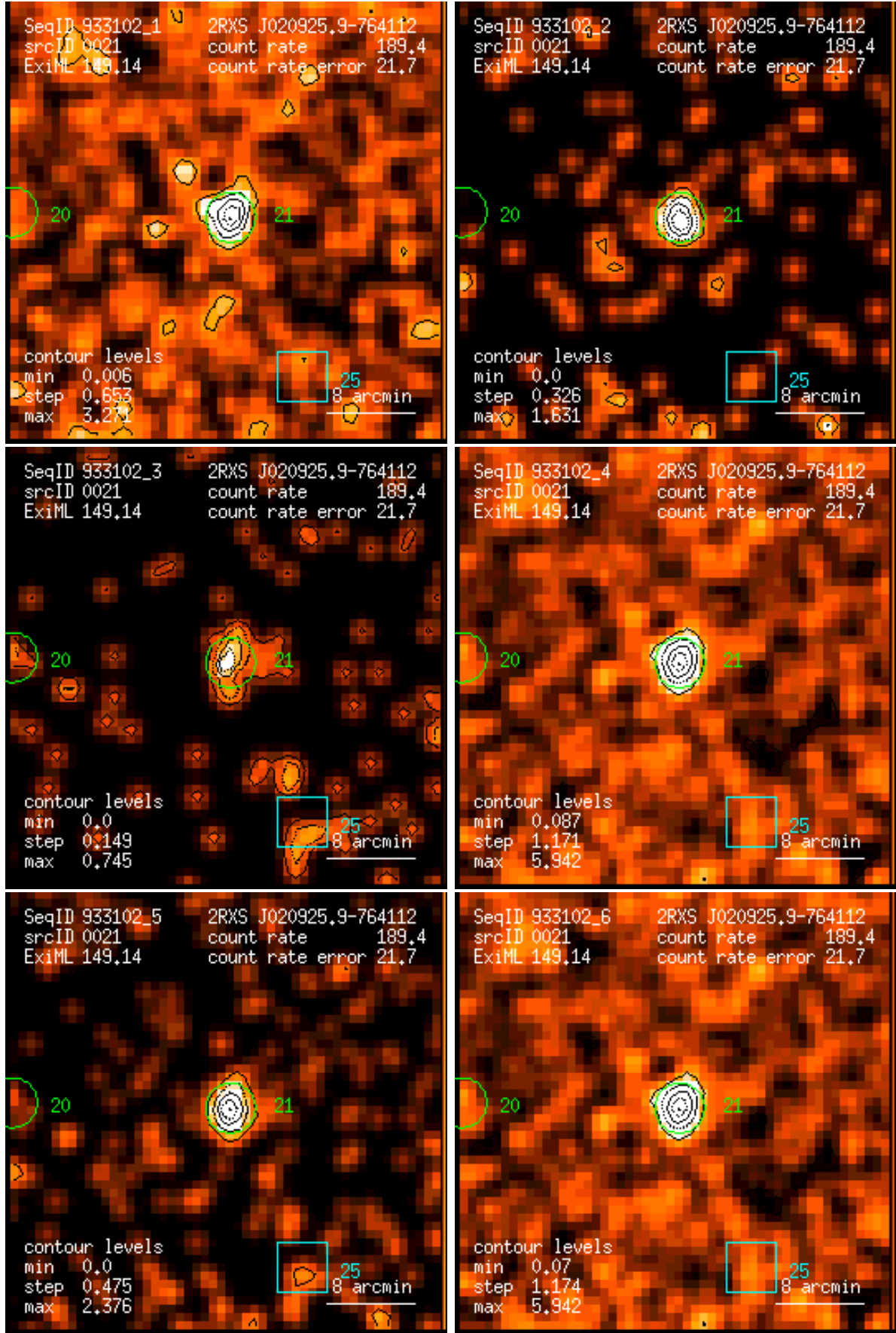
Figure 21: RASS 933102: detection 0021: band rate images, Gaussian filter: (1) PSPC channels 11 – 41, (2) 52 – 90, (3) 91 – 201, (4) 11 – 235, (5) 52 – 201, (6) 11 – 201. Broad band rates in counts/ks. Band rate contour levels in counts/ks/arcmin 2 .
