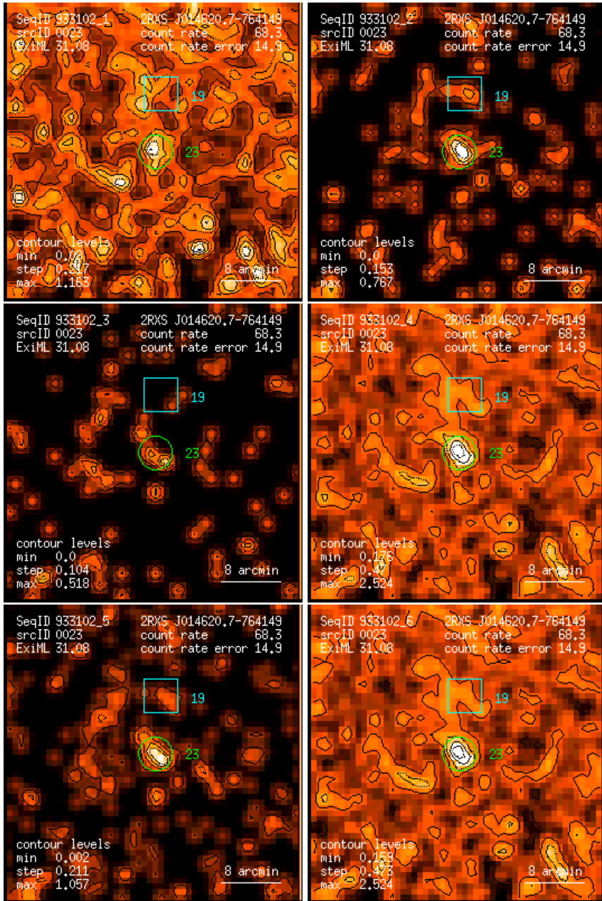
Figure 23: RASS 933102: detection 0023: band rate images, Gaussian filter: (1) PSPC channels 11 – 41, (2) 52 – 90, (3) 91 – 201, (4) 11 – 235, (5) 52 – 201, (6) 11 – 201. Broad band rates in counts/ks. Band rate contour levels in counts/ks/arcmin 2 .
