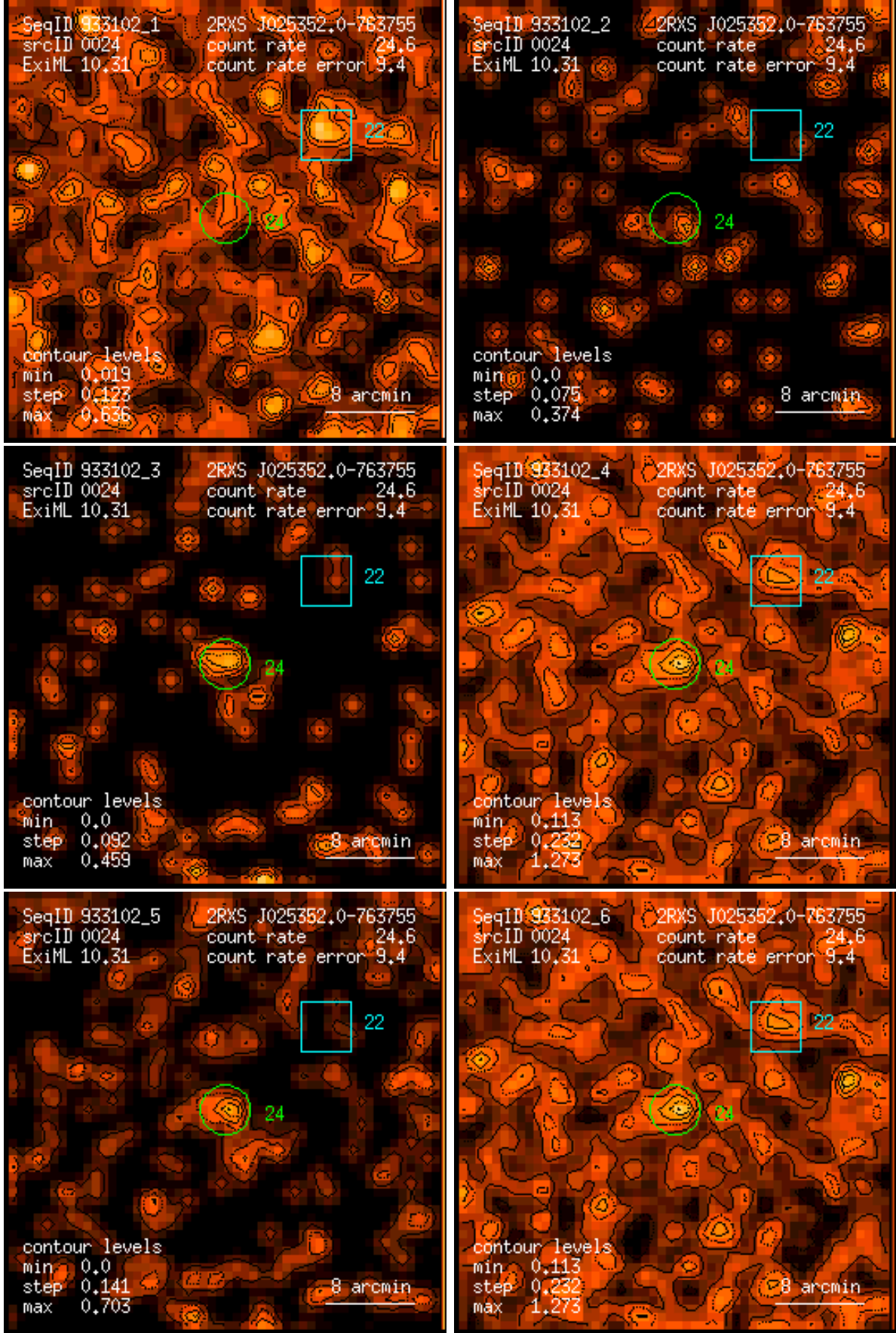
Figure 24: RASS 933102: detection 0024: band rate images, Gaussian filter: (1) PSPC channels 11 – 41, (2) 52 – 90, (3) 91 – 201, (4) 11 – 235, (5) 52 – 201, (6) 11 – 201. Broad band rates in counts/ks. Band rate contour levels in counts/ks/arcmin 2 .
