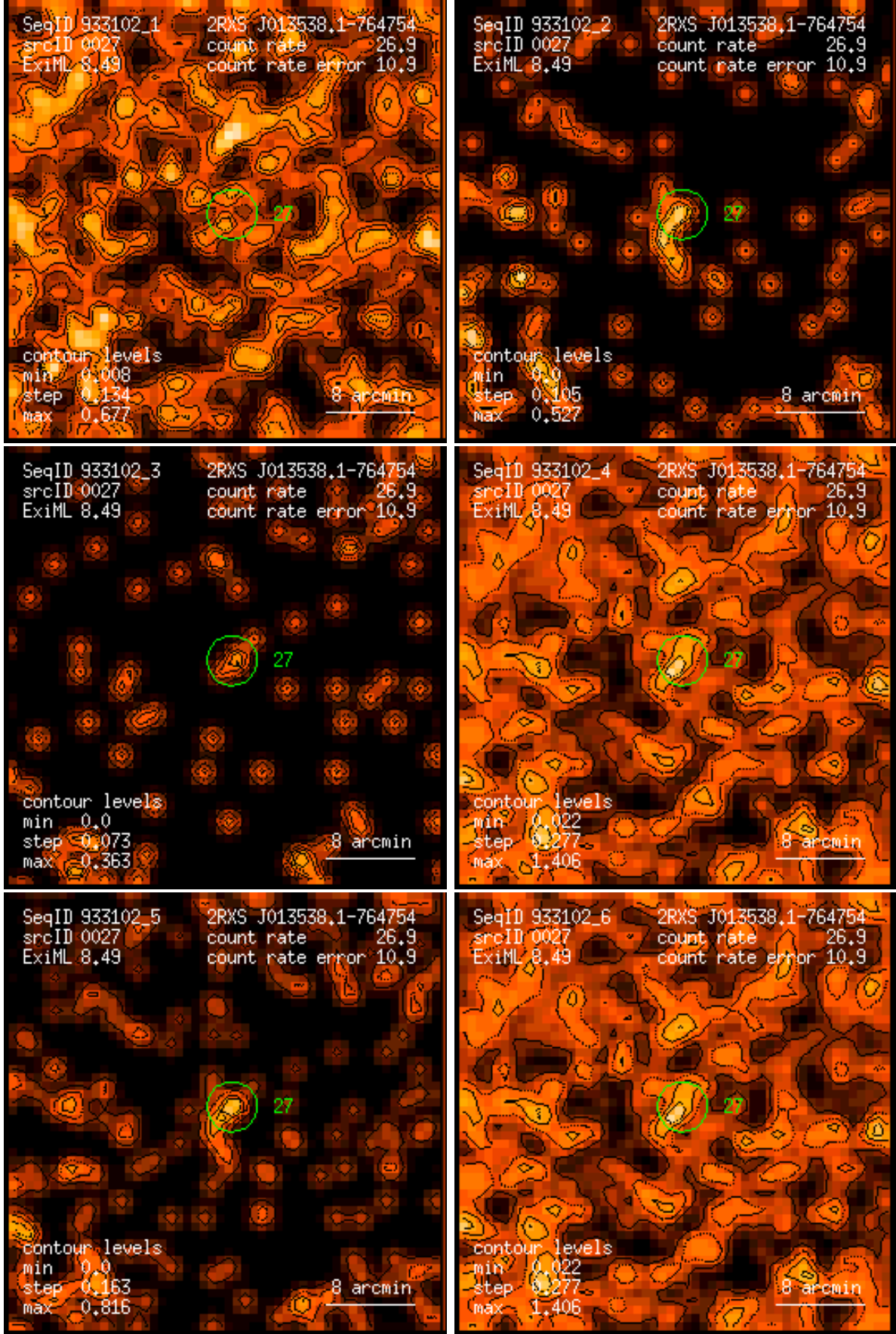
Figure 27: RASS 933102: detection 0027: band rate images, Gaussian filter: (1) PSPC channels 11 – 41, (2) 52 – 90, (3) 91 – 201, (4) 11 – 235, (5) 52 – 201, (6) 11 – 201. Broad band rates in counts/ks. Band rate contour levels in counts/ks/arcmin 2 .
