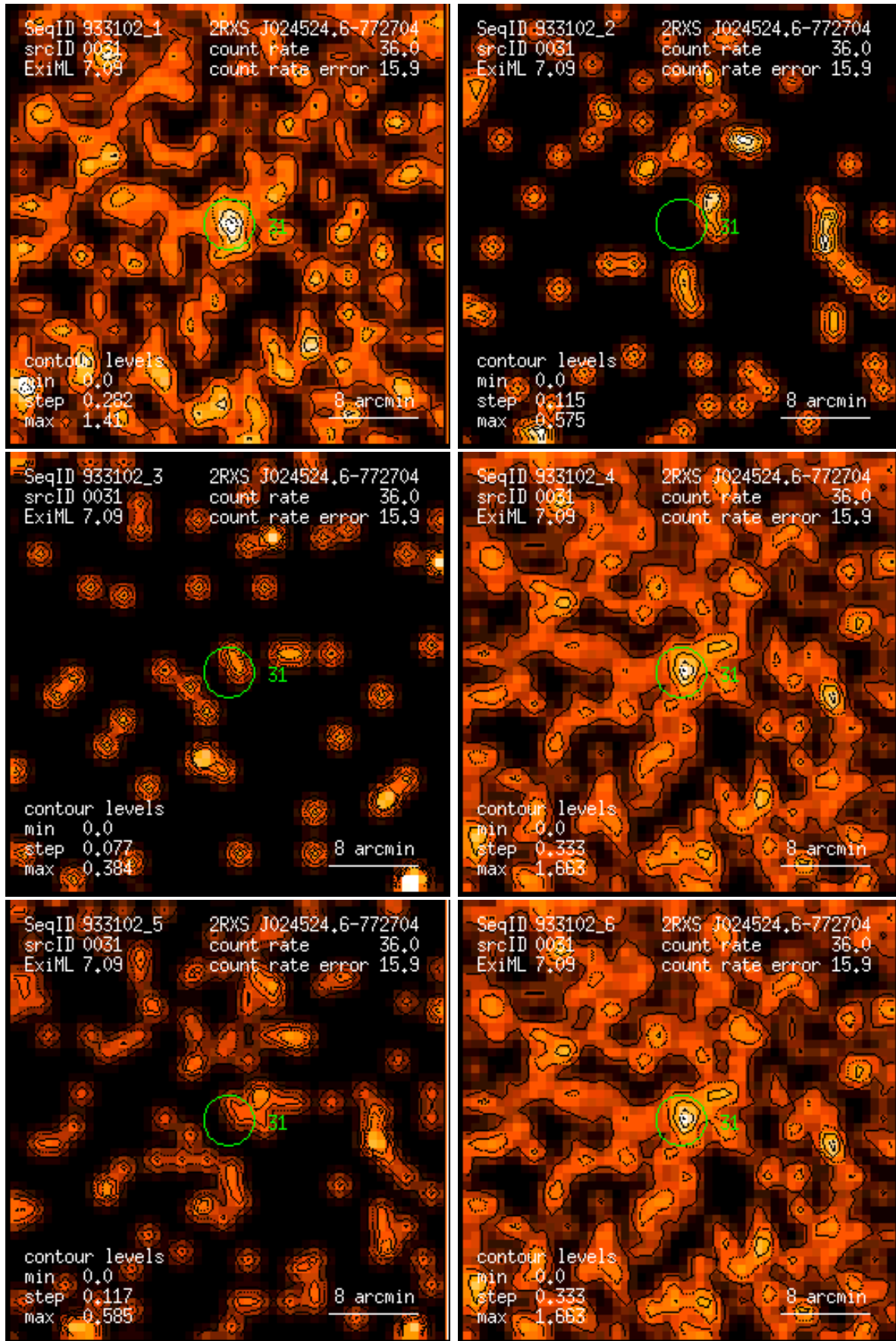
Figure 31: RASS 933102: detection 0031: band rate images, Gaussian filter: (1) PSPC channels 11 – 41, (2) 52 – 90, (3) 91 – 201, (4) 11 – 235, (5) 52 – 201, (6) 11 – 201. Broad band rates in counts/ks. Band rate contour levels in counts/ks/arcmin 2 .
