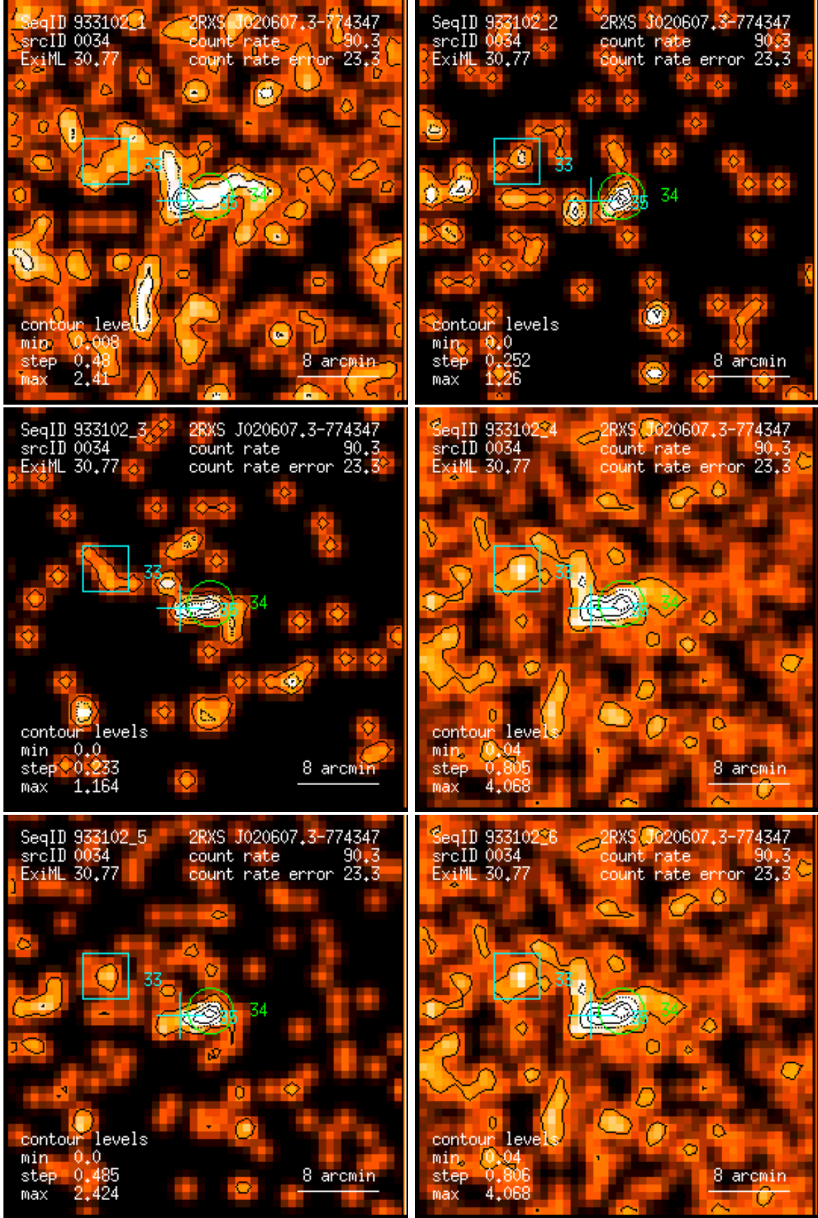
Figure 34: RASS 933102: detection 0034: band rate images, Gaussian filter: (1) PSPC channels 11 – 41, (2) 52 – 90, (3) 91 – 201, (4) 11 – 235, (5) 52 – 201, (6) 11 – 201. Broad band rates in counts/ks. Band rate contour levels in counts/ks/arcmin 2 .
