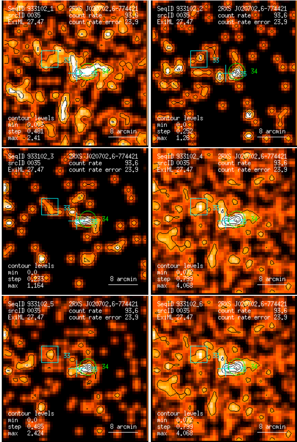
Figure 35: RASS 933102: detection 0035: band rate images, Gaussian filter: (1) PSPC channels 11 – 41, (2) 52 – 90, (3) 91 – 201, (4) 11 – 235, (5) 52 – 201, (6) 11 – 201. Broad band rates in counts/ks. Band rate contour levels in counts/ks/arcmin 2 .
