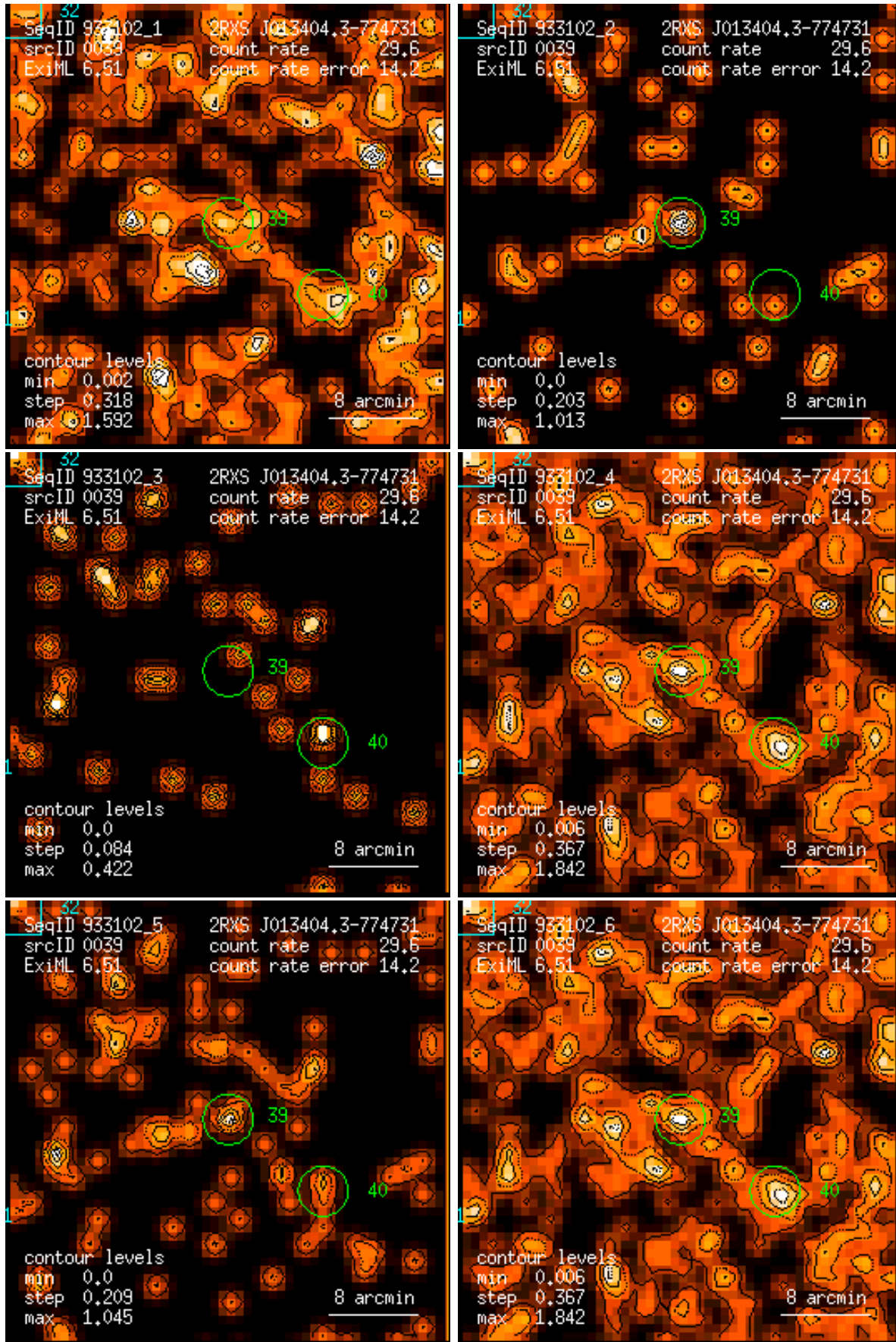
Figure 39: RASS 933102: detection 0039: band rate images, Gaussian filter: (1) PSPC channels 11 – 41, (2) 52 – 90, (3) 91 – 201, (4) 11 – 235, (5) 52 – 201, (6) 11 – 201. Broad band rates in counts/ks. Band rate contour levels in counts/ks/arcmin 2 .
