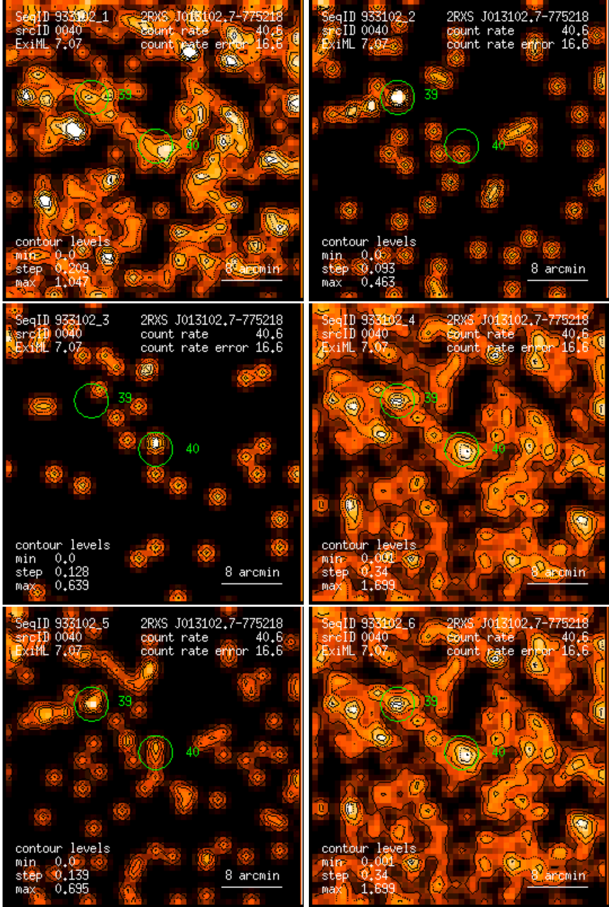
Figure 40: RASS 933102: detection 0040: band rate images, Gaussian filter: (1) PSPC channels 11 – 41, (2) 52 – 90, (3) 91 – 201, (4) 11 – 235, (5) 52 – 201, (6) 11 – 201. Broad band rates in counts/ks. Band rate contour levels in counts/ks/arcmin 2 .
